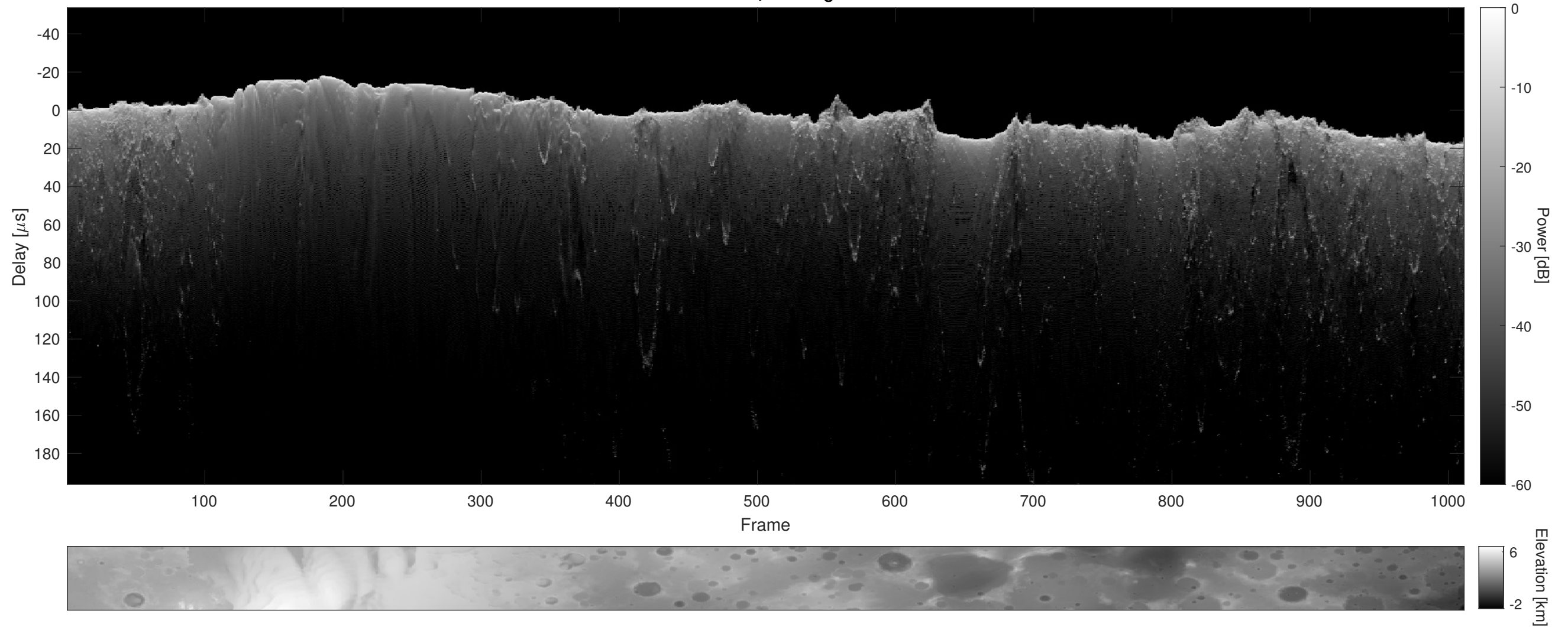
Orbit 10628, Cluttergram
