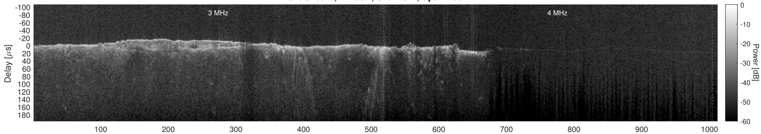
Orbit 10628, Cluttergram
