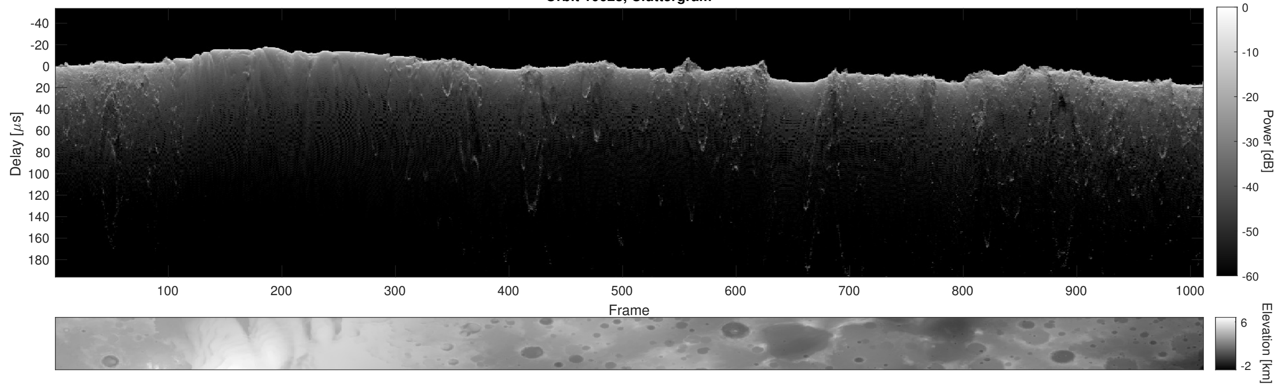
Orbit 10628, Cluttergram
