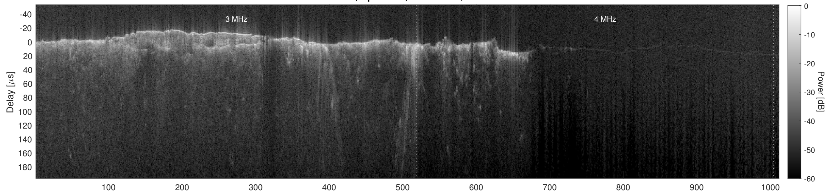
Orbit 10628, Cluttergram
