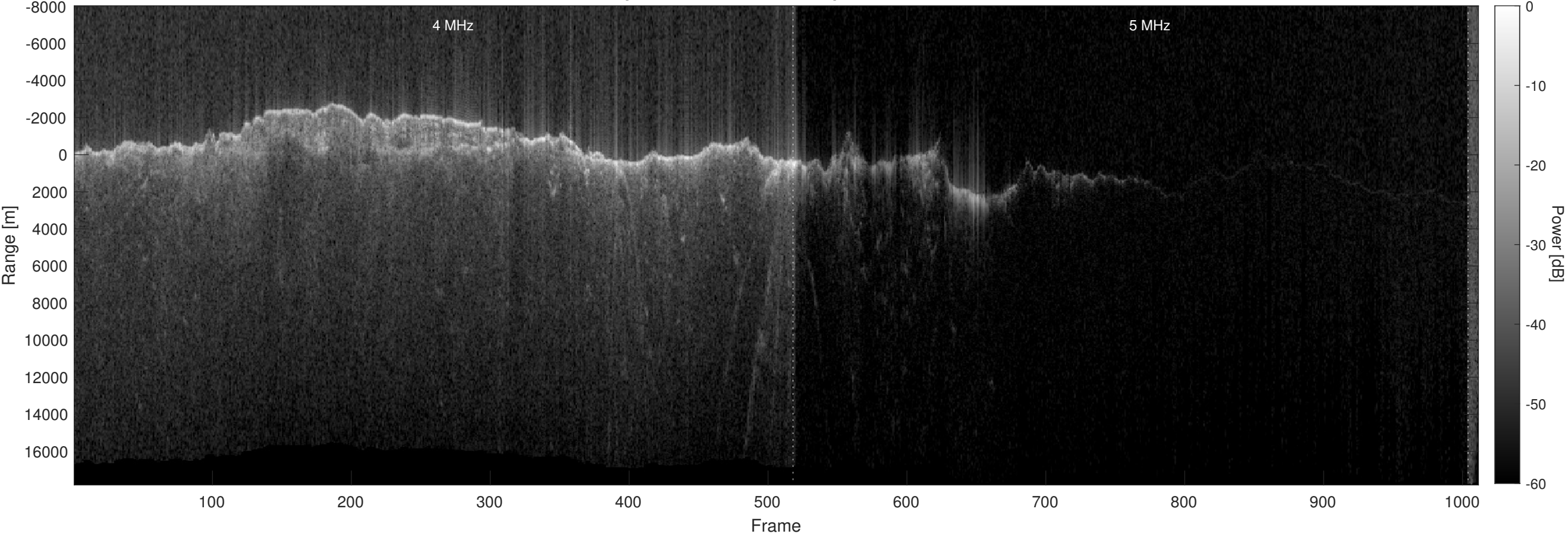
Orbit 10628, Optimized, No Window, Depth-Corrected, Channel 2
