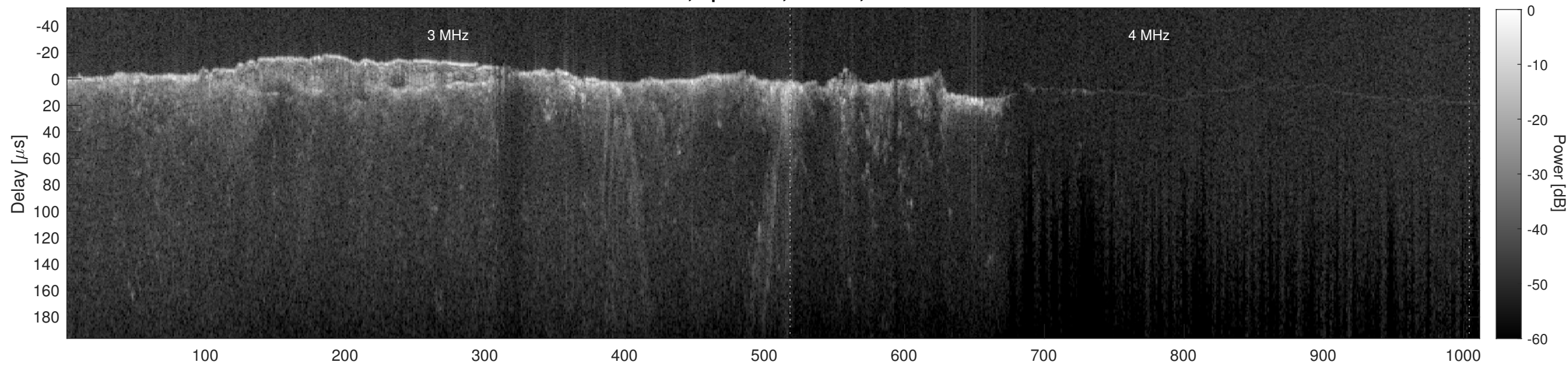
Orbit 10628, Cluttergram
