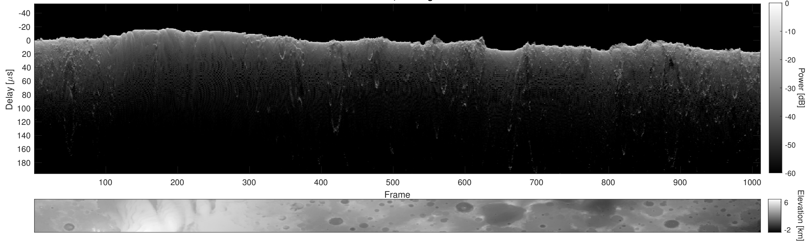
Orbit 10628, Cluttergram
