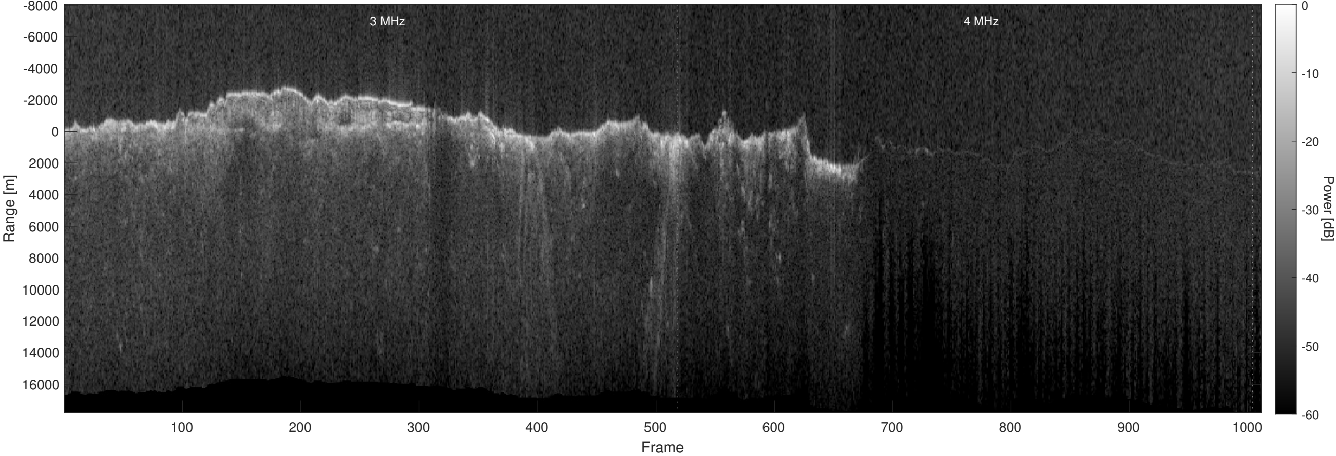
Orbit 10628, Optimized, Window, Depth-Corrected, Channel 2
