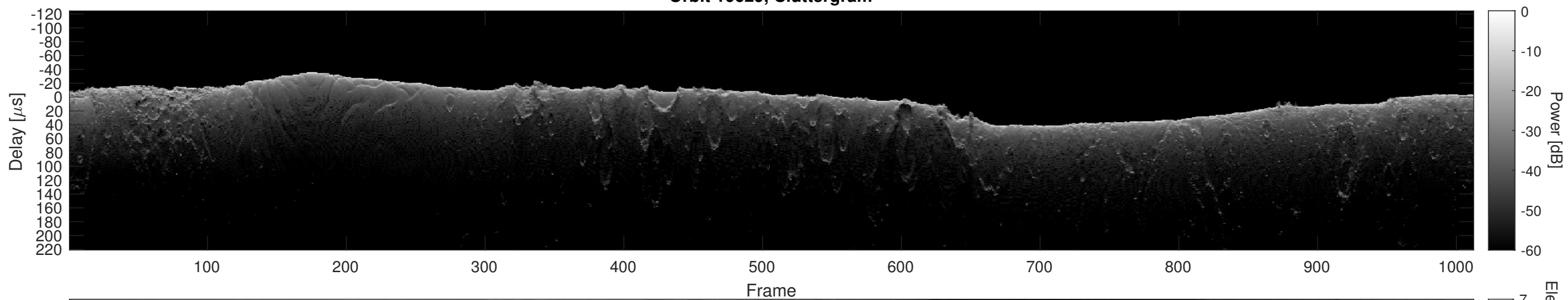
Orbit 10629, Cluttergram
