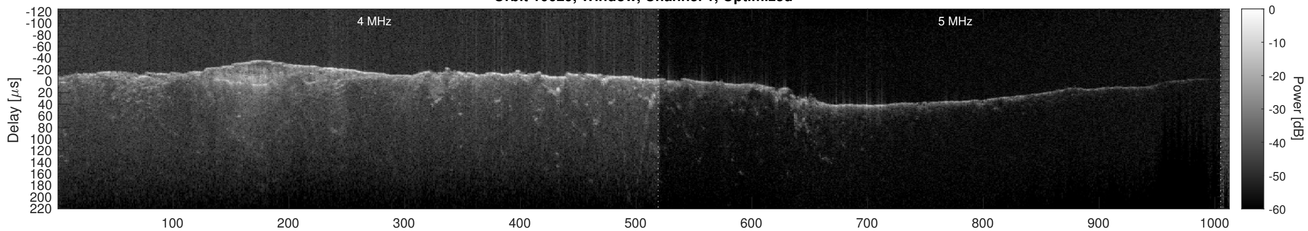
Orbit 10629, Cluttergram
