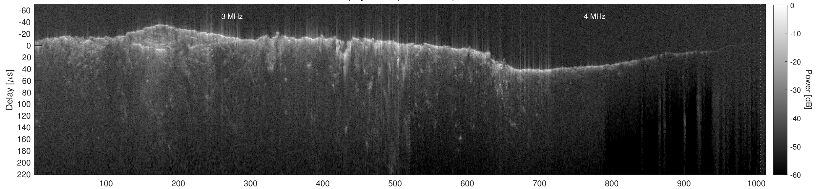
Orbit 10629, Cluttergram
