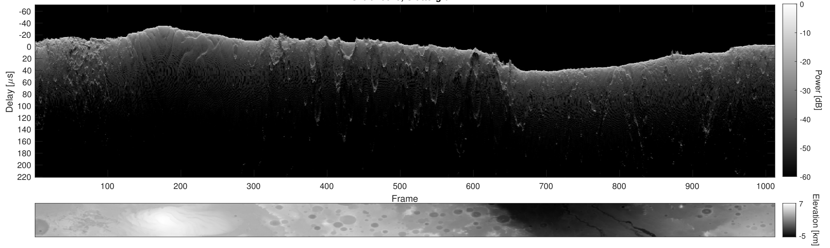
Orbit 10629, Cluttergram
