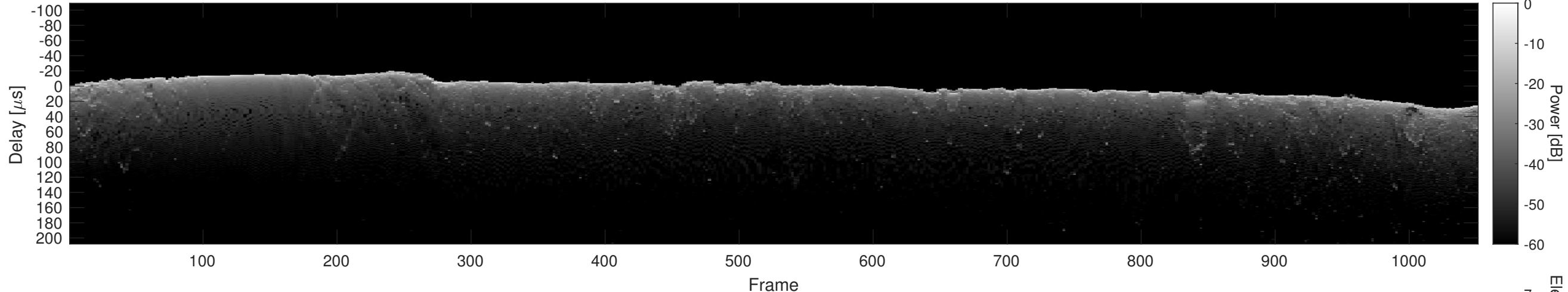
Orbit 10630, Cluttergram
