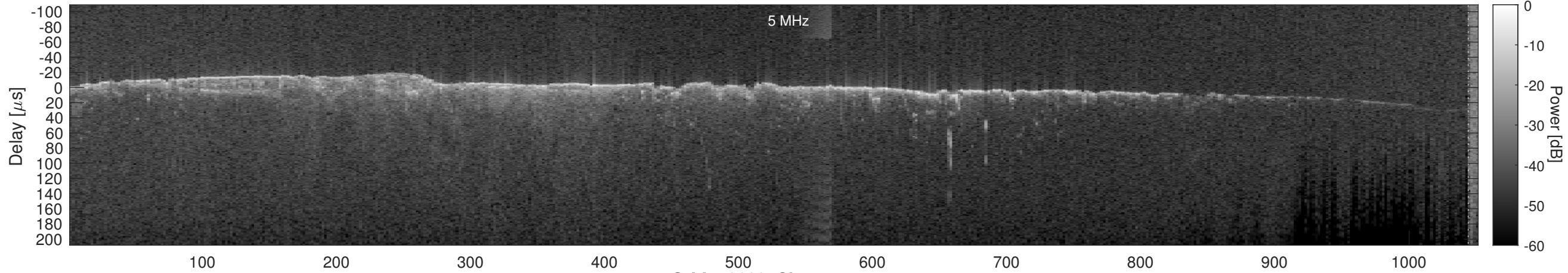
Orbit 10630, Cluttergram
