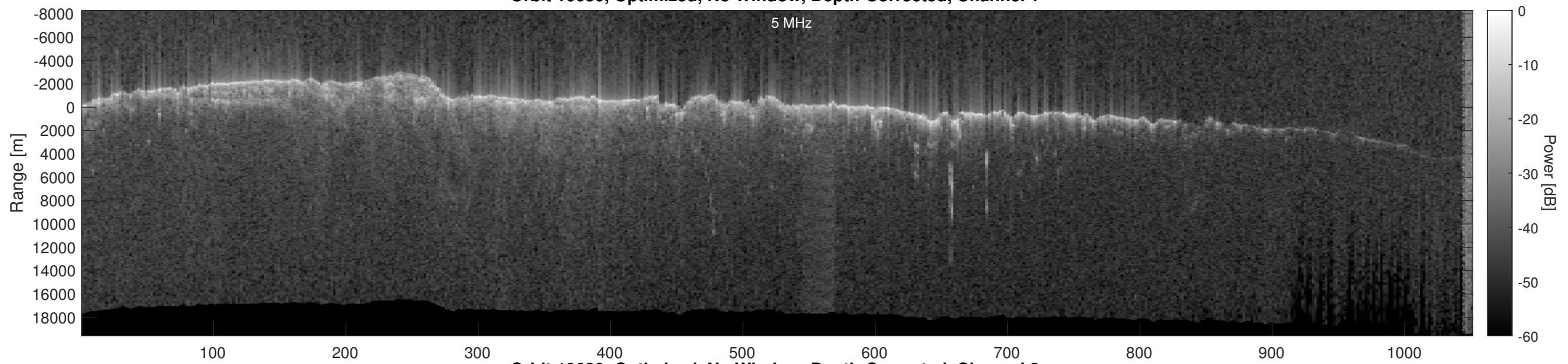
Orbit 10630, Optimized, No Window, Depth-Corrected, Channel 2
