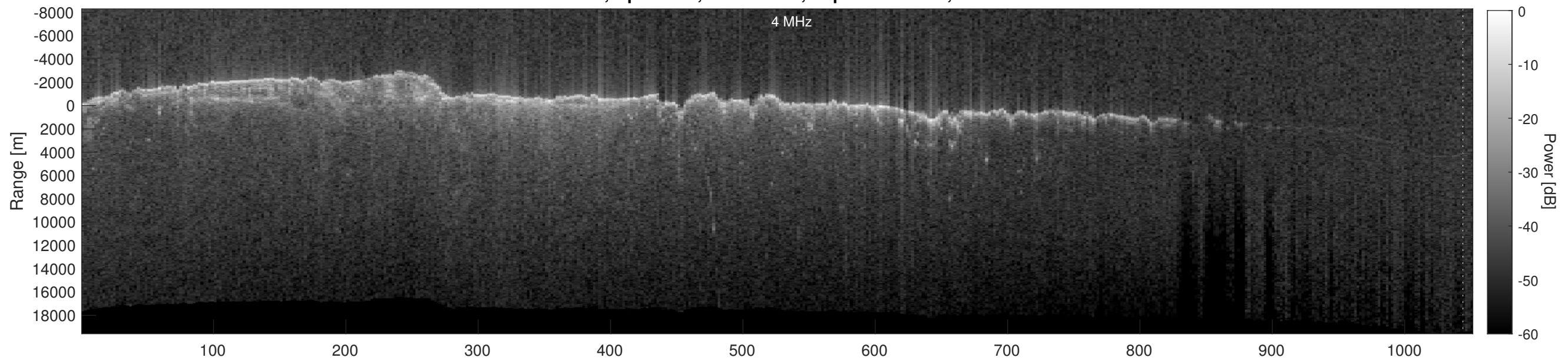
Orbit 10630, Depth-Corrected Cluttergram
