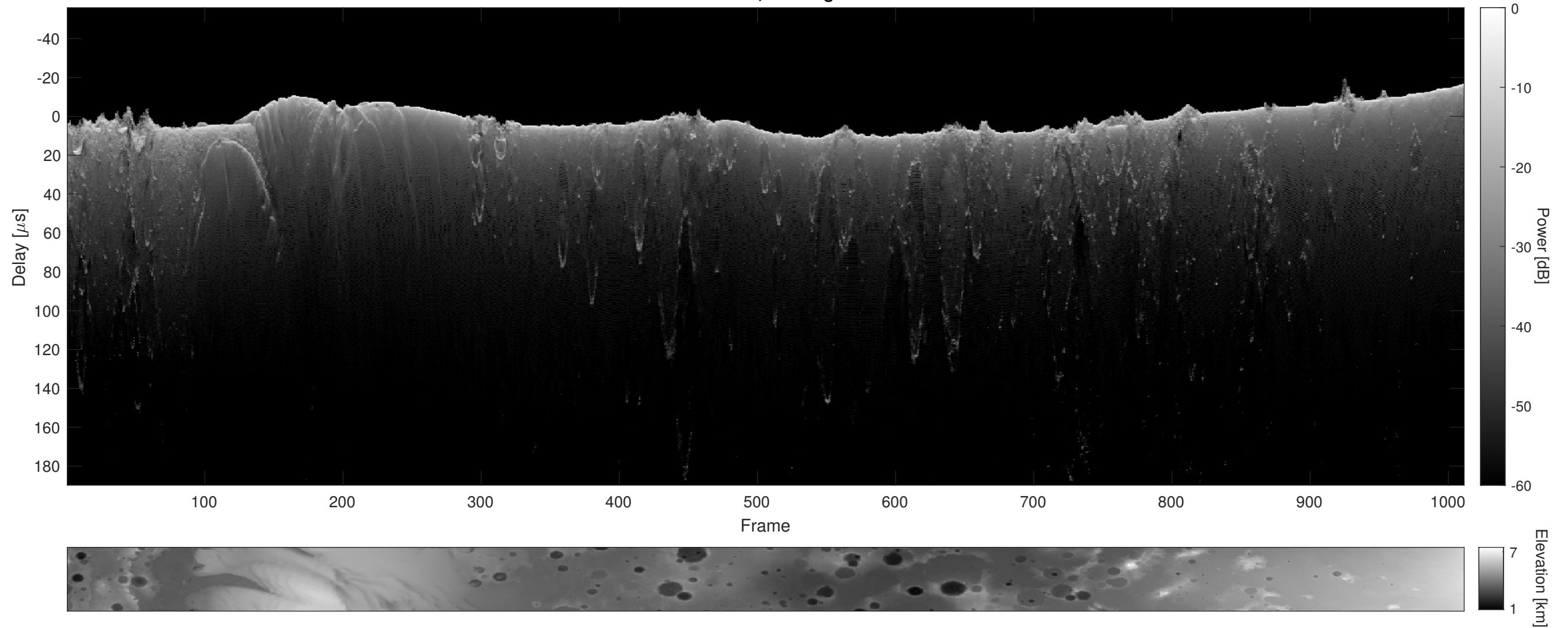
Orbit 10631, Cluttergram
