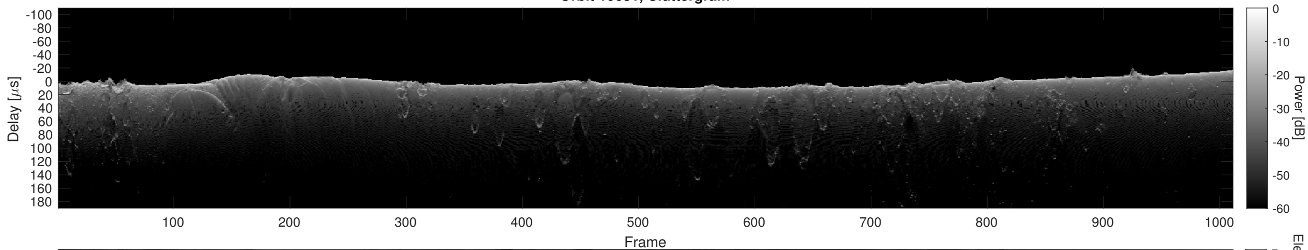
Orbit 10631, Cluttergram
