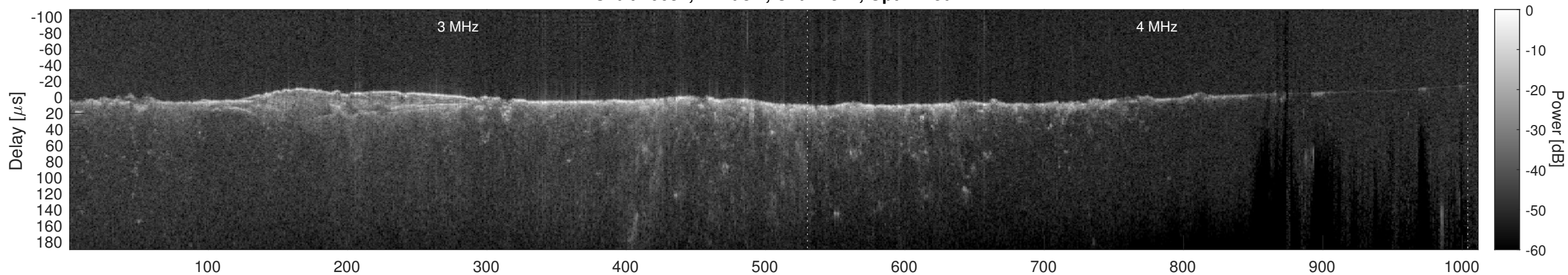
Orbit 10631, Cluttergram
