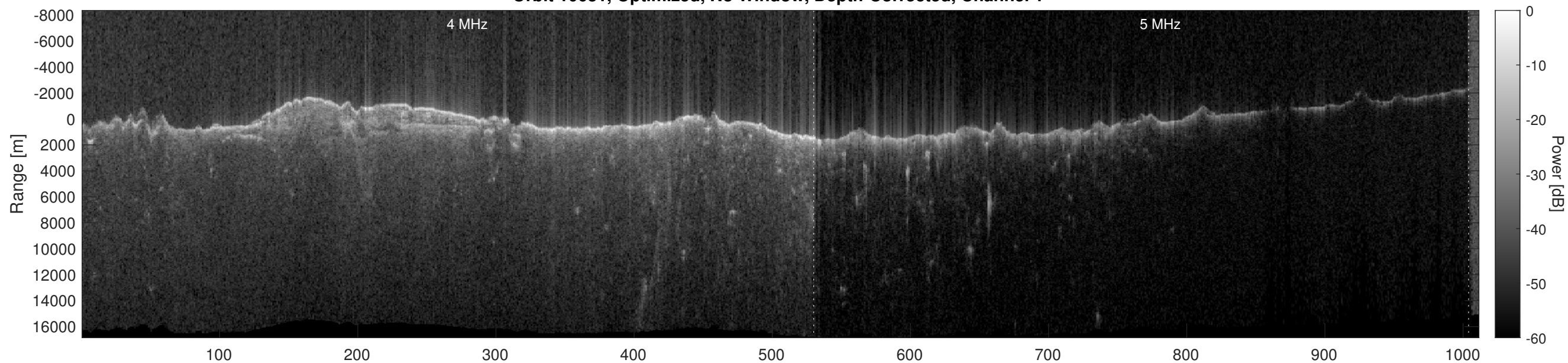
Orbit 10631, Optimized, No Window, Depth-Corrected, Channel 2
