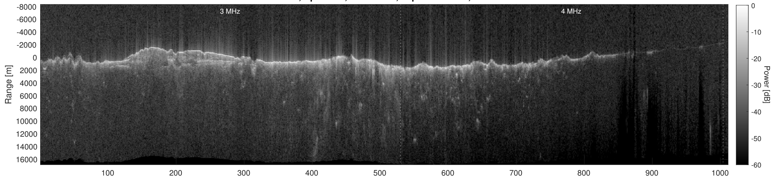
Orbit 10631, Depth-Corrected Cluttergram
