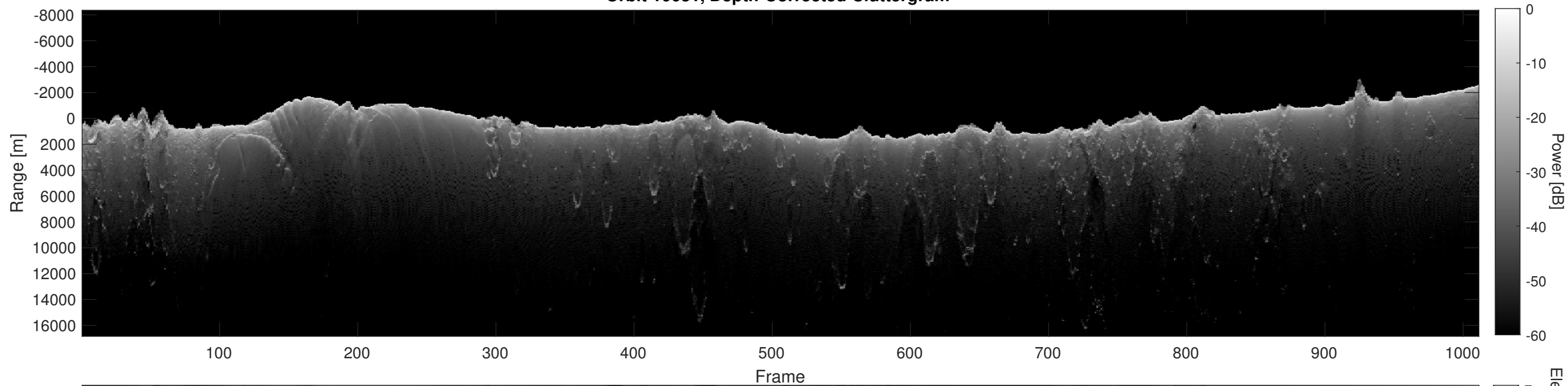
Orbit 10631, Depth-Corrected Cluttergram
