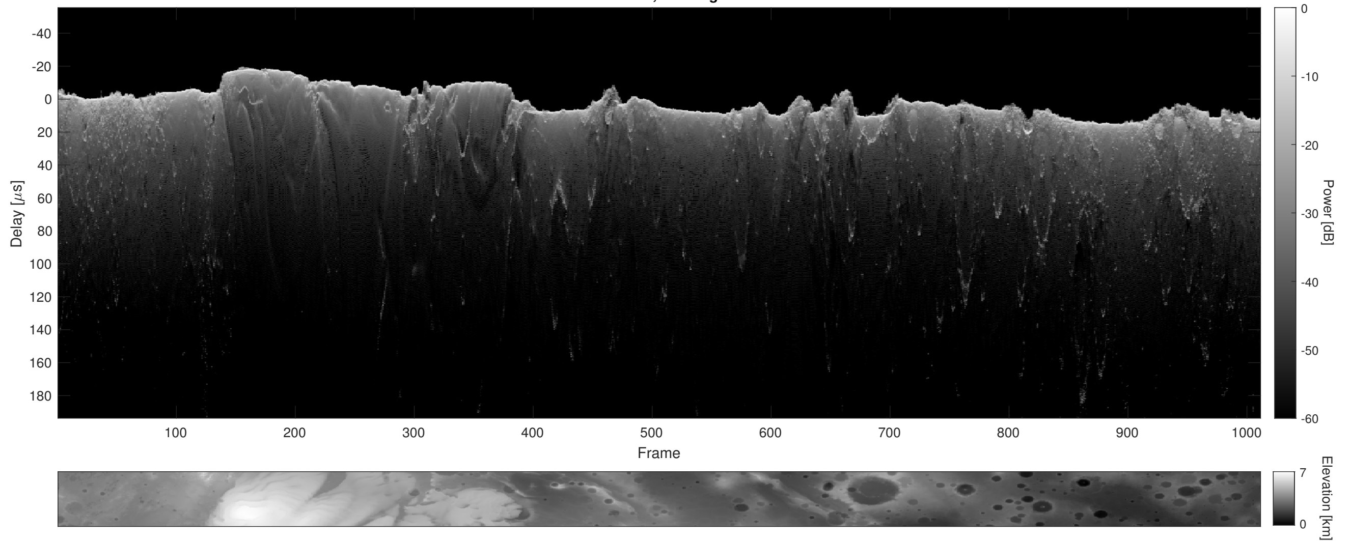
Orbit 10632, Cluttergram
