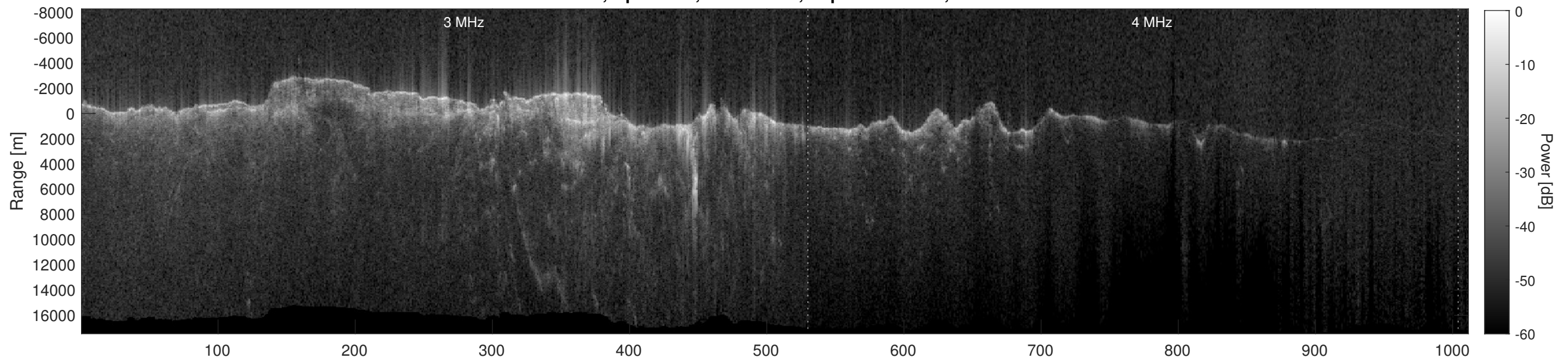
Orbit 10632, Depth-Corrected Cluttergram
