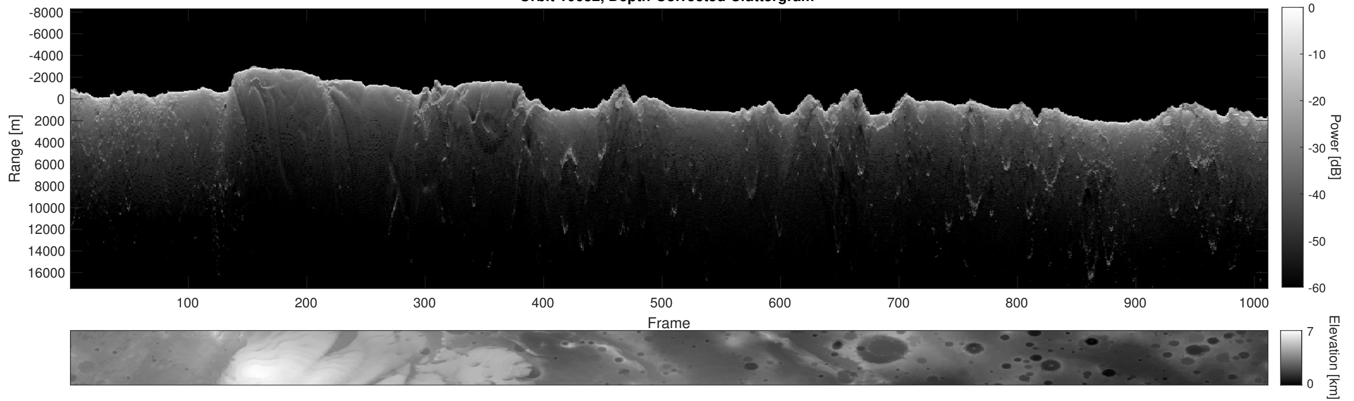
Orbit 10632, Depth-Corrected Cluttergram
