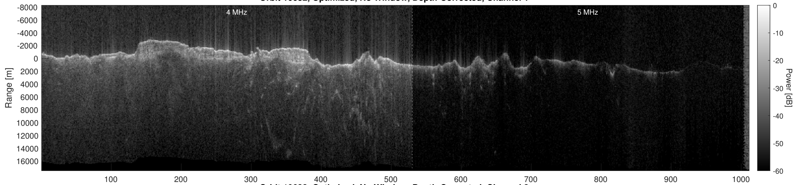
Orbit 10632, Optimized, No Window, Depth-Corrected, Channel 2
