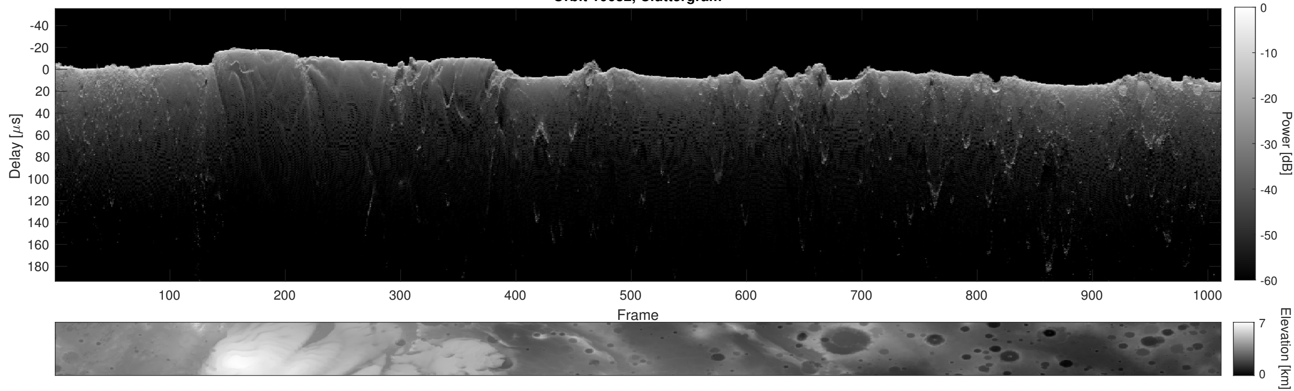
Orbit 10632, Cluttergram
