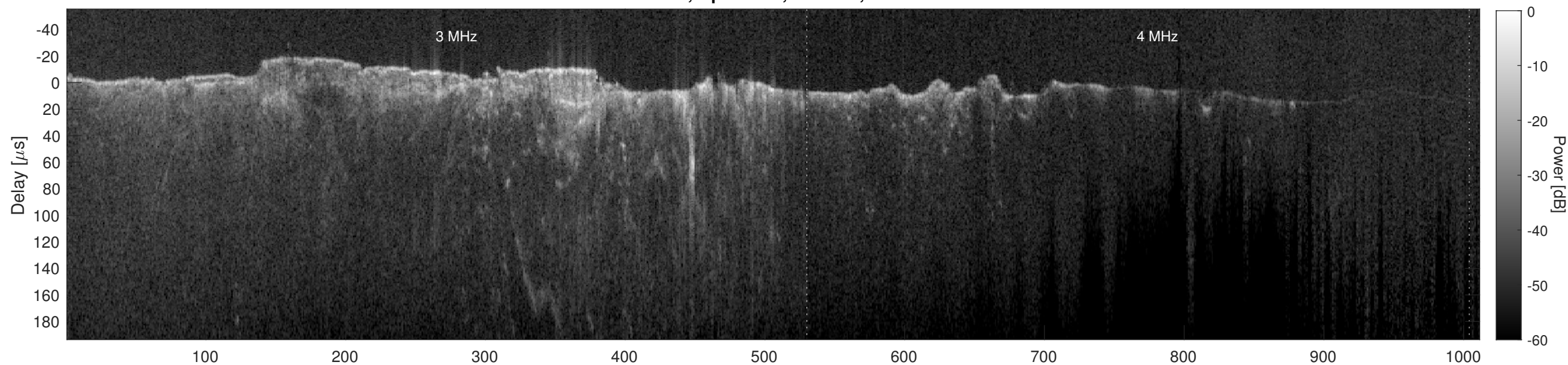
Orbit 10632, Cluttergram
