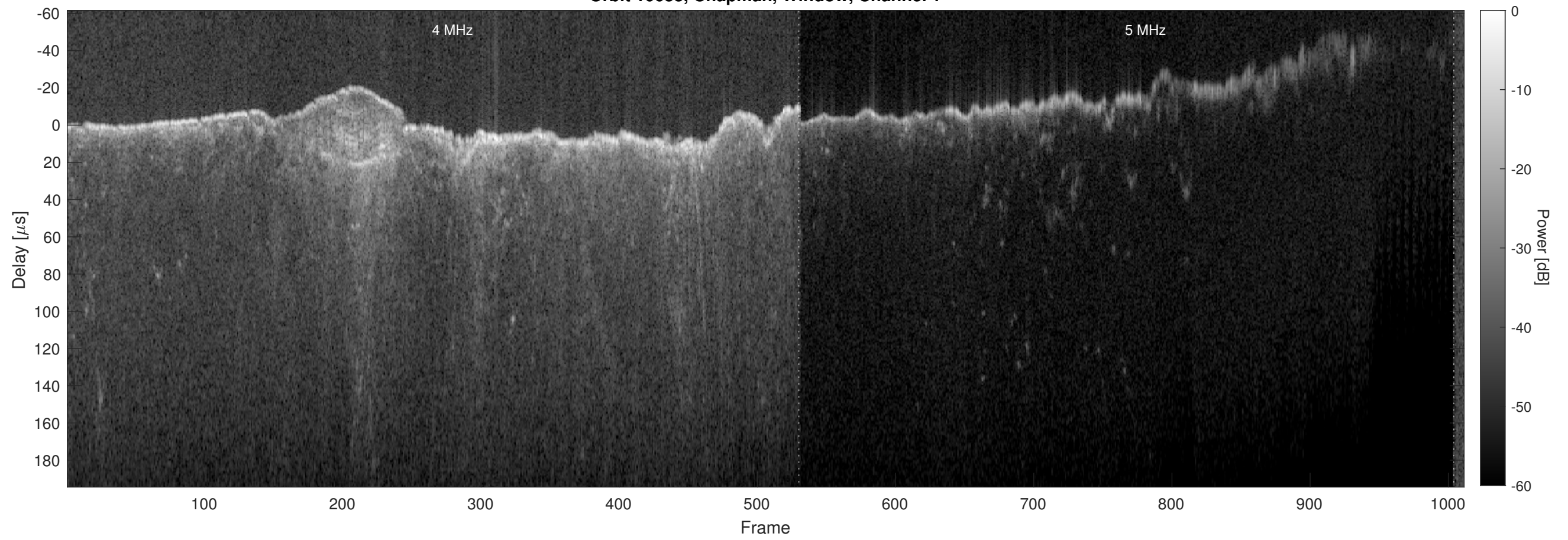
Orbit 10633, Chapman, Window, Channel 2
