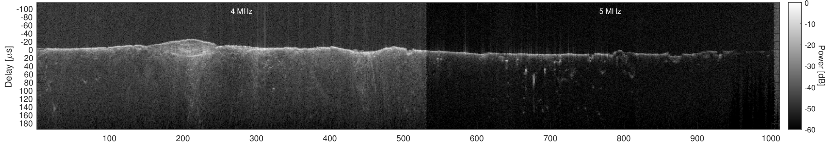
Orbit 10633, Cluttergram
