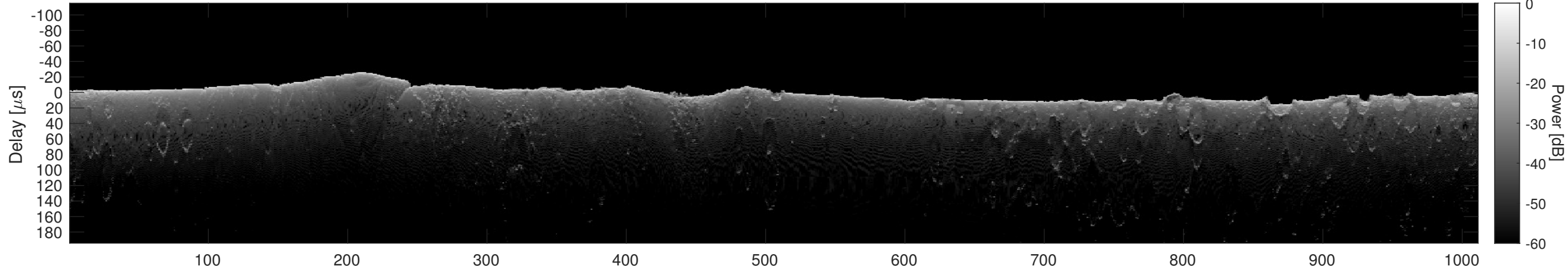
Orbit 10633, Cluttergram
