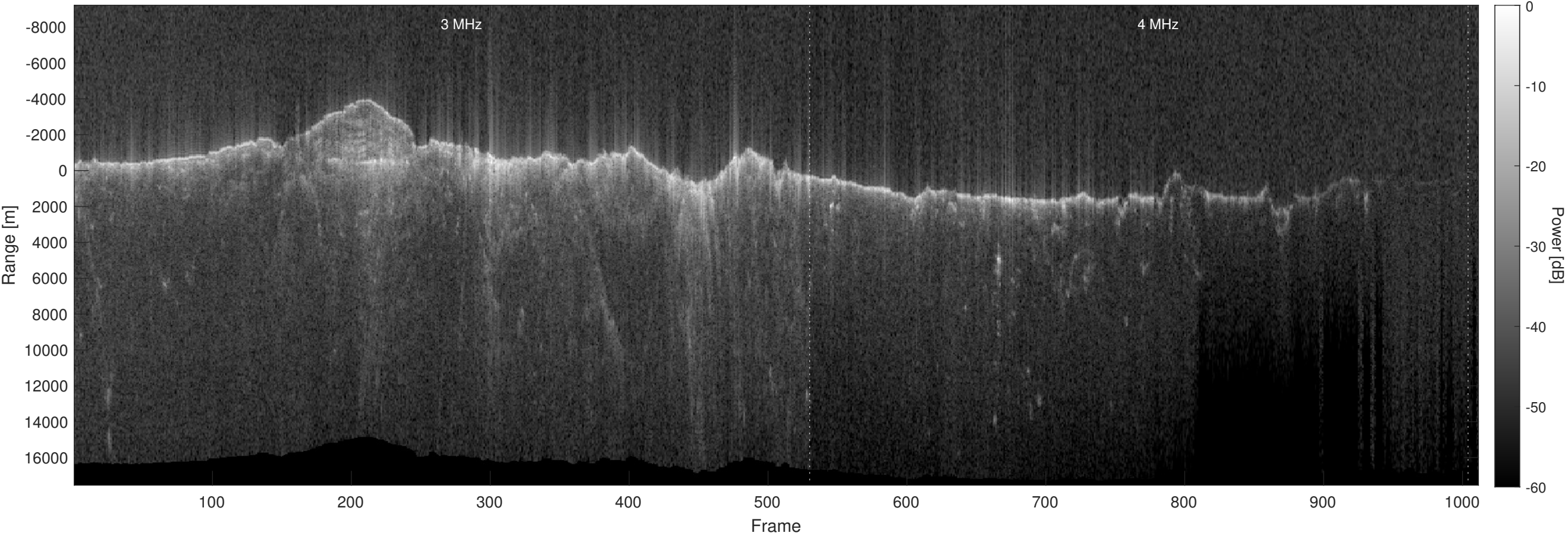
Orbit 10633, Optimized, No Window, Depth-Corrected, Channel 2
