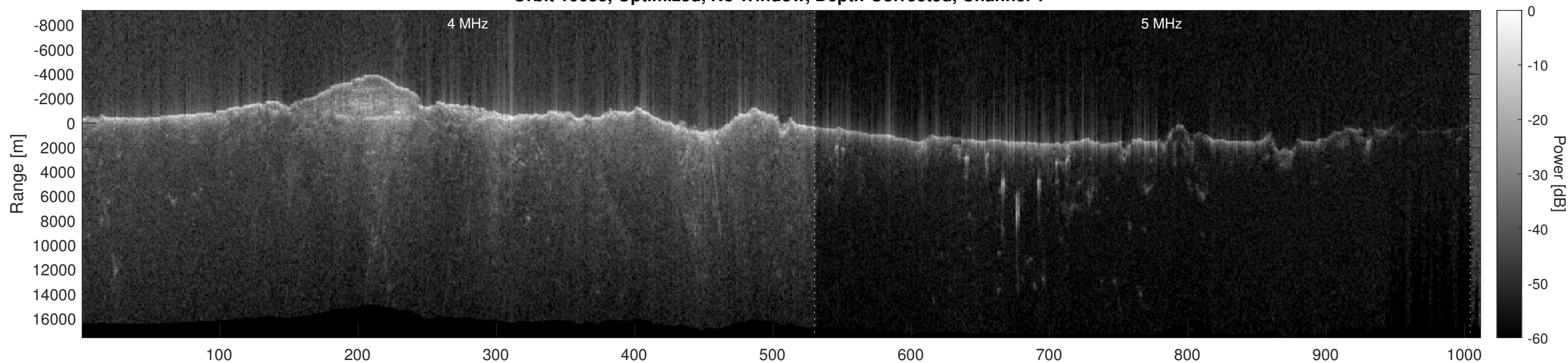
Orbit 10633, Optimized, No Window, Depth-Corrected, Channel 2
