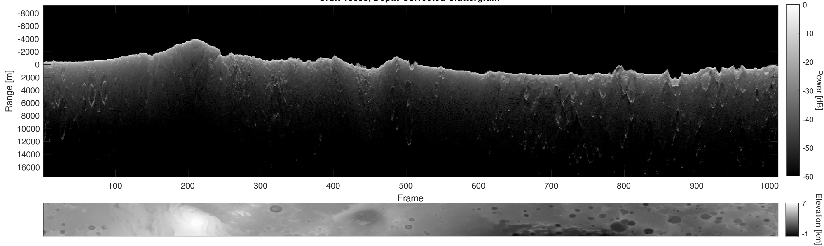
Orbit 10633, Depth-Corrected Cluttergram
