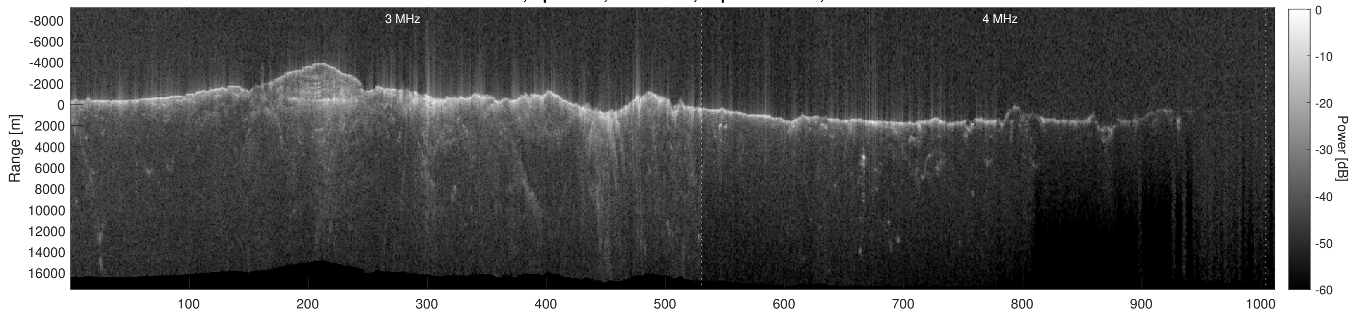
Orbit 10633, Depth-Corrected Cluttergram
