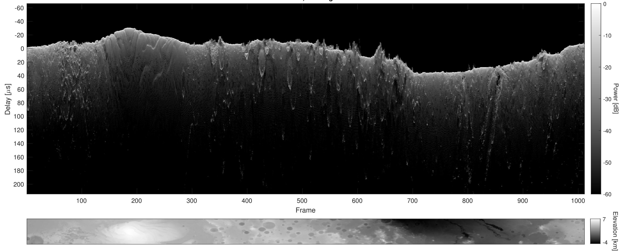
Orbit 10636, Cluttergram
