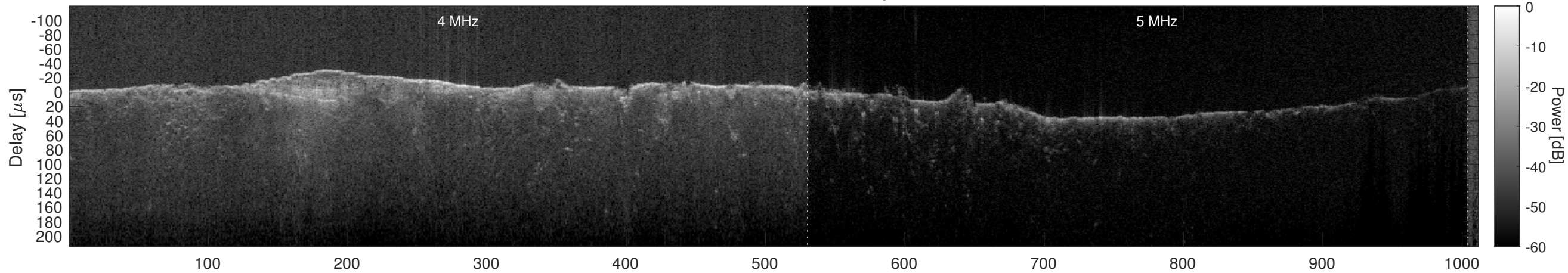
Orbit 10636, Cluttergram
