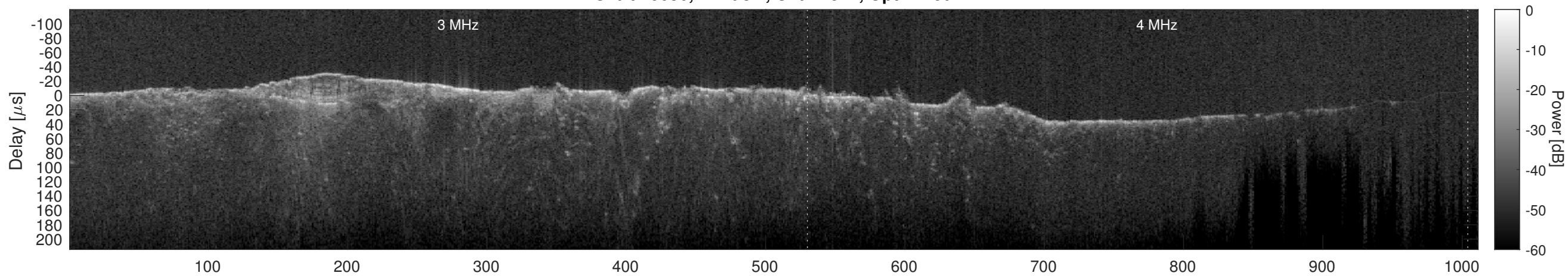
Orbit 10636, Cluttergram
