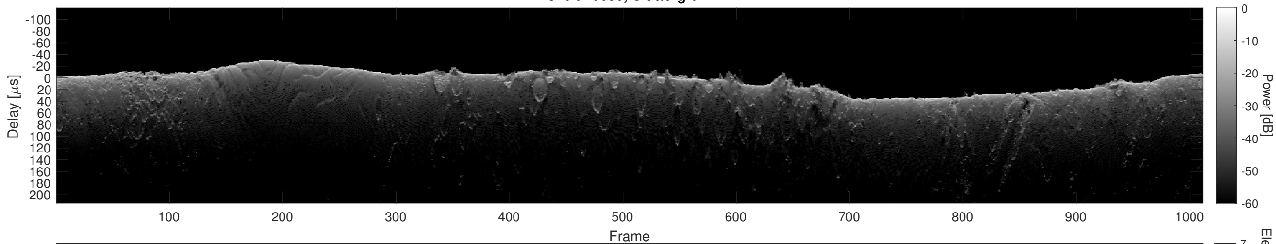
Orbit 10636, Cluttergram
