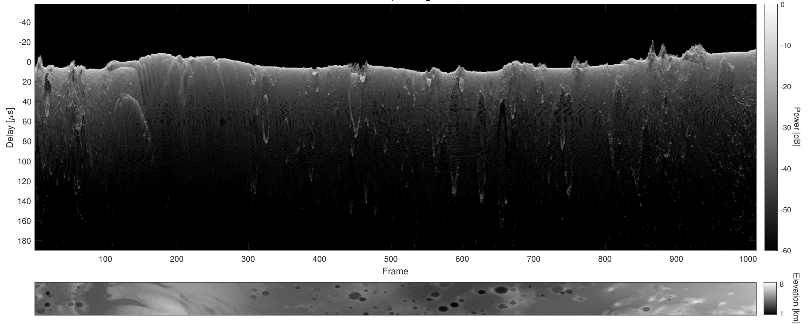
Orbit 10638, Cluttergram
