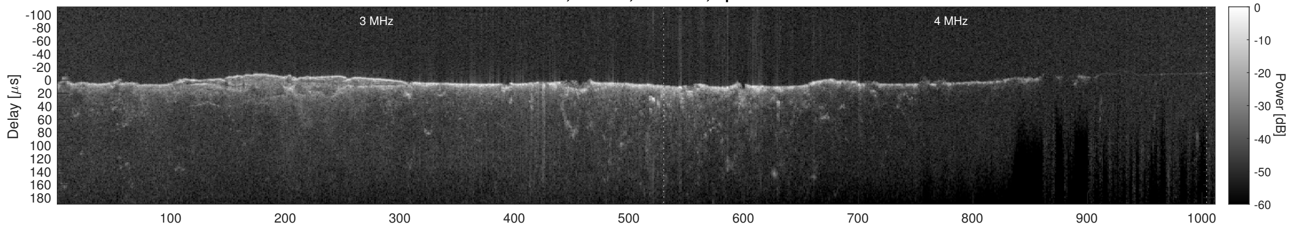
Orbit 10638, Cluttergram
