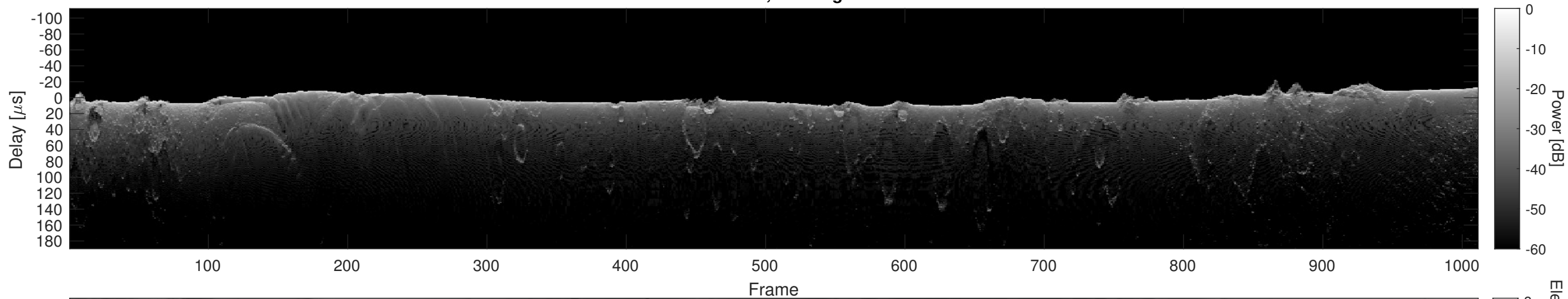
Orbit 10638, Cluttergram
