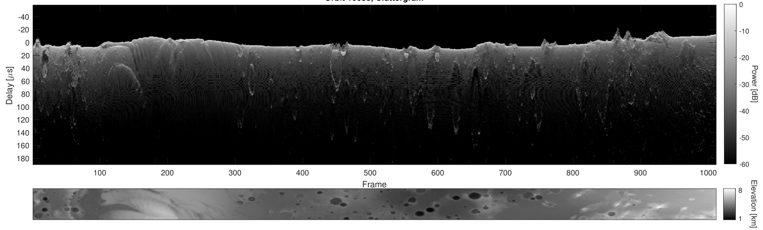
Orbit 10638, Cluttergram
