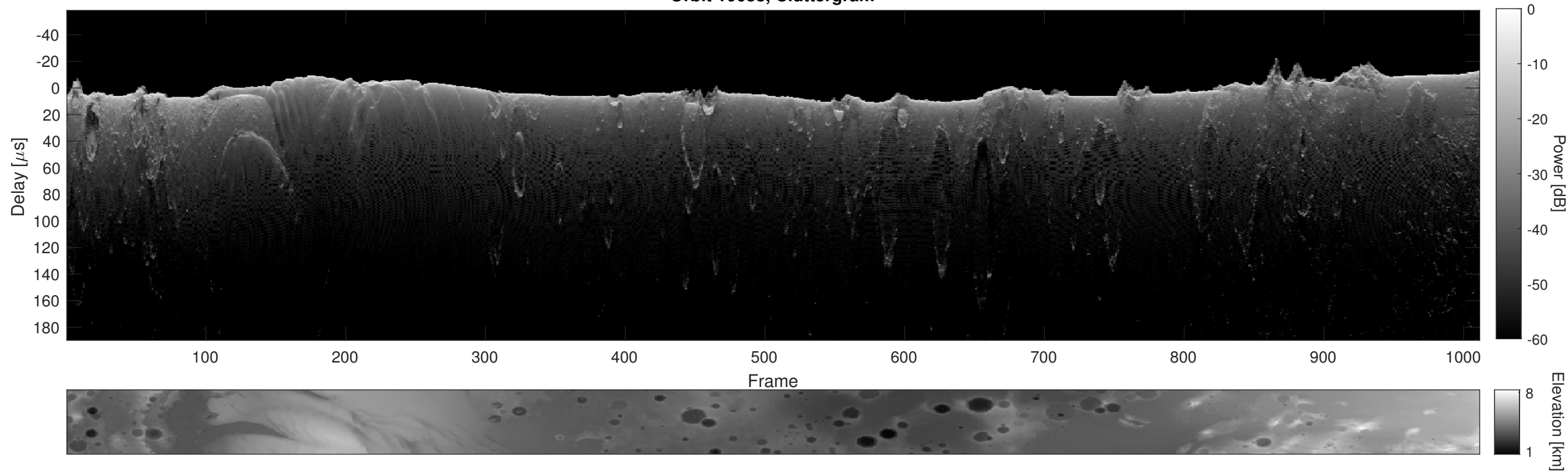
Orbit 10638, Cluttergram
