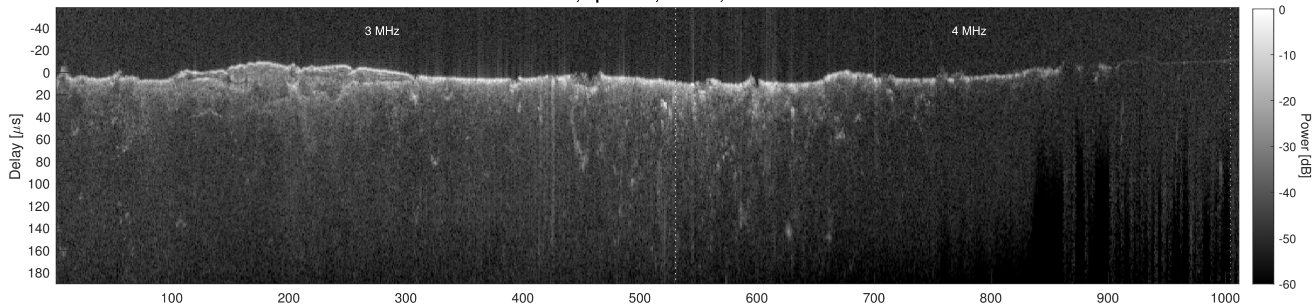
Orbit 10638, Cluttergram
