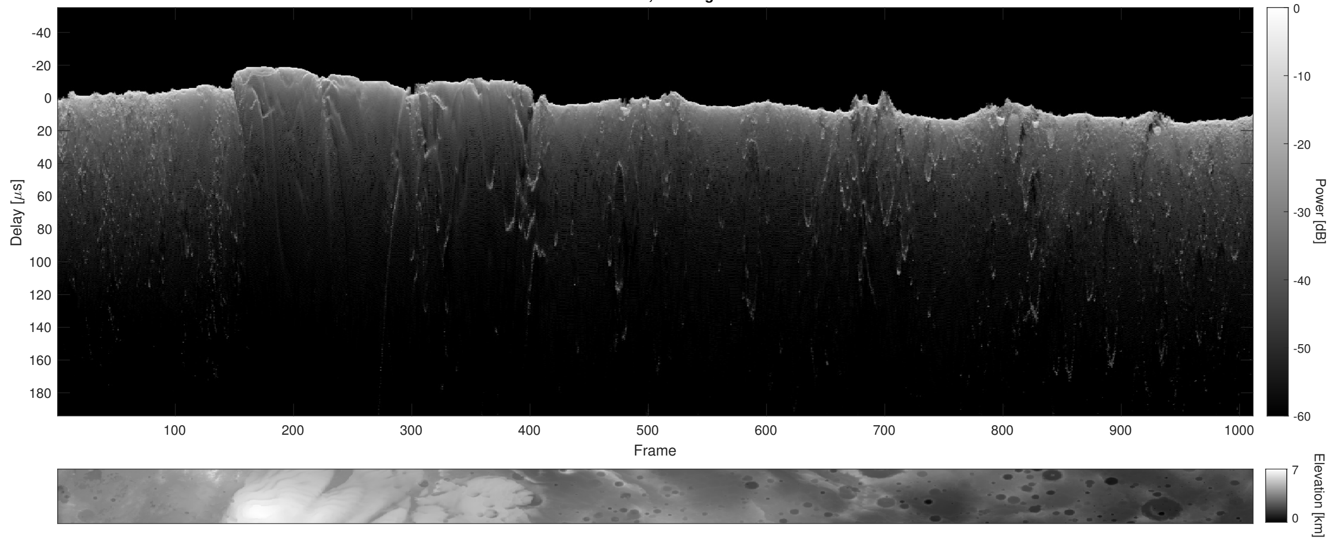
Orbit 10639, Cluttergram
