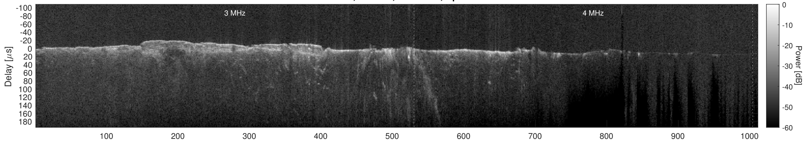
Orbit 10639, Cluttergram
