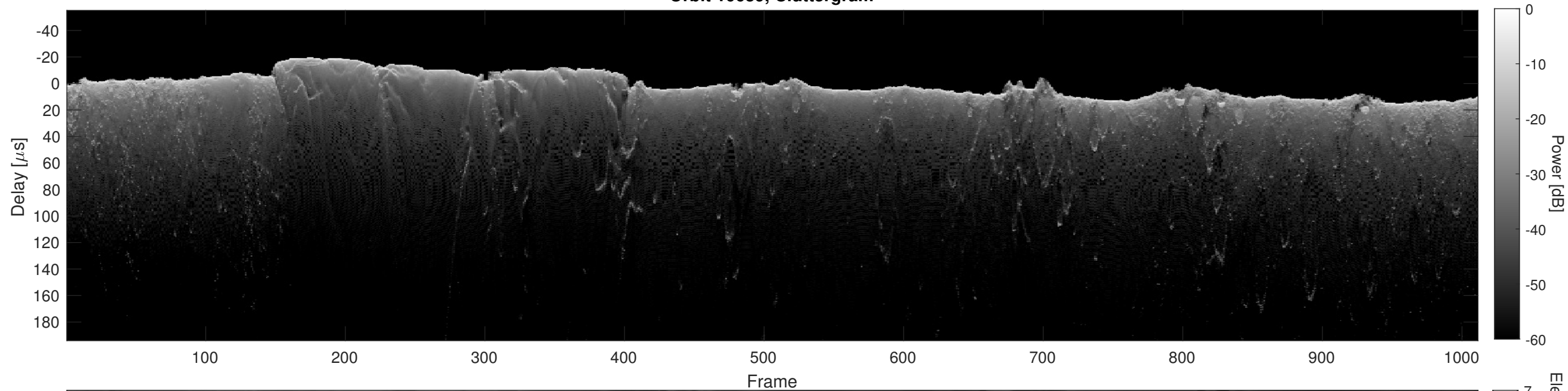
Orbit 10639, Cluttergram
