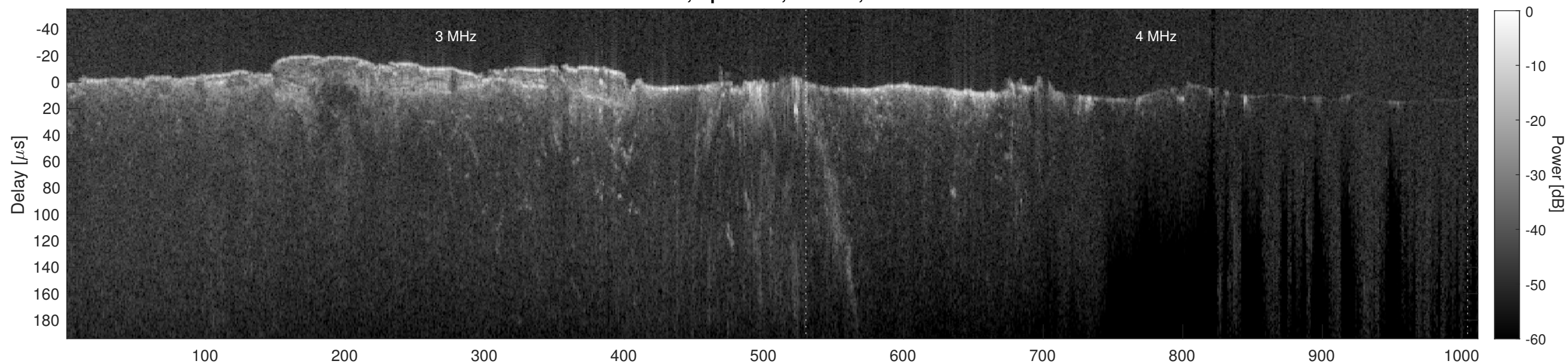
Orbit 10639, Cluttergram
