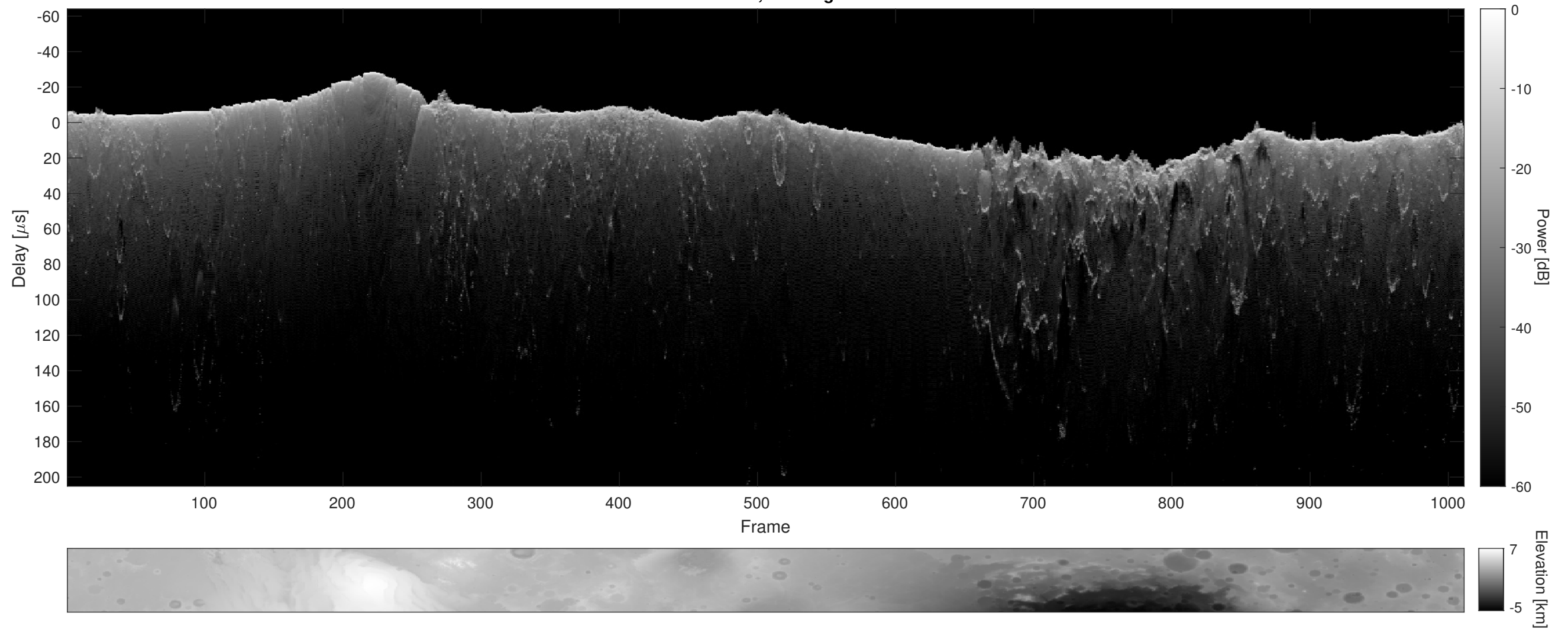
Orbit 10640, Cluttergram
