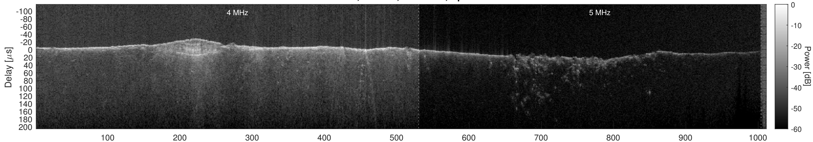
Orbit 10640, Cluttergram
