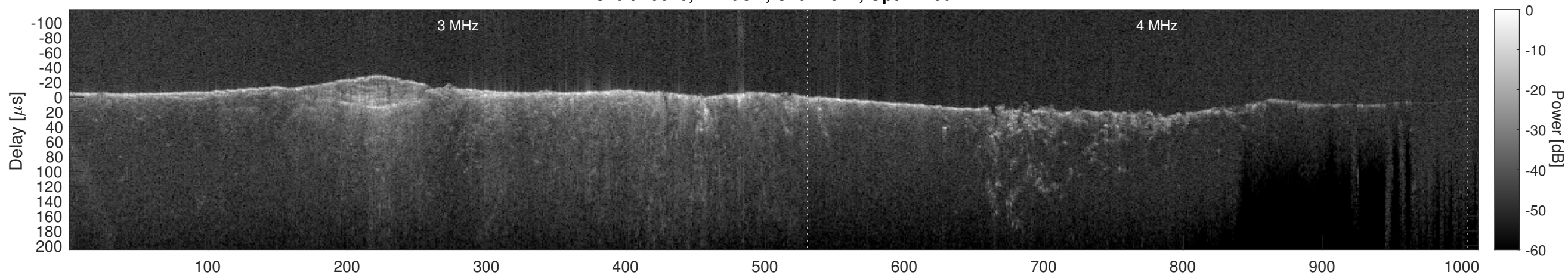
Orbit 10640, Cluttergram
