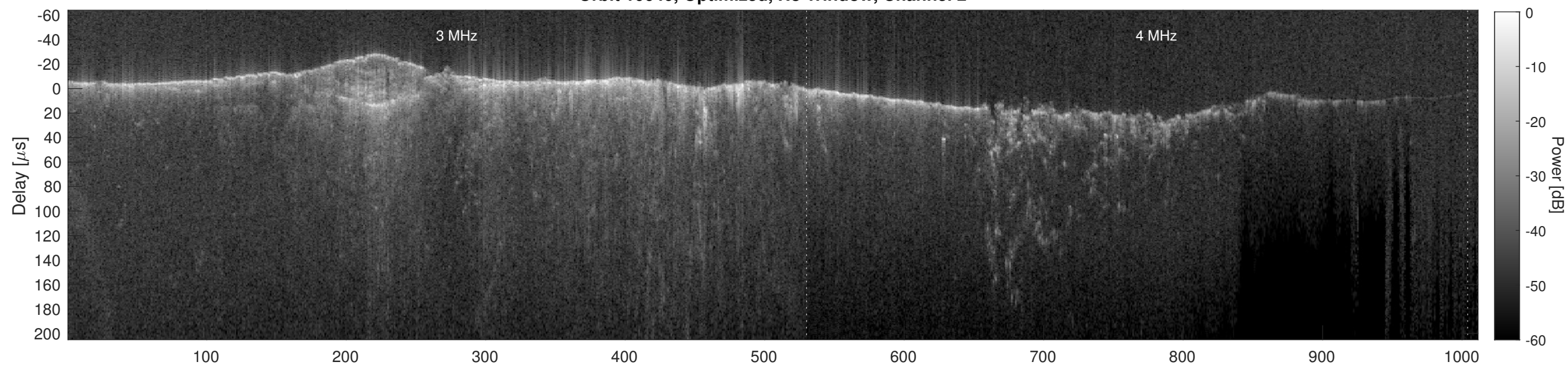
Orbit 10640, Cluttergram
