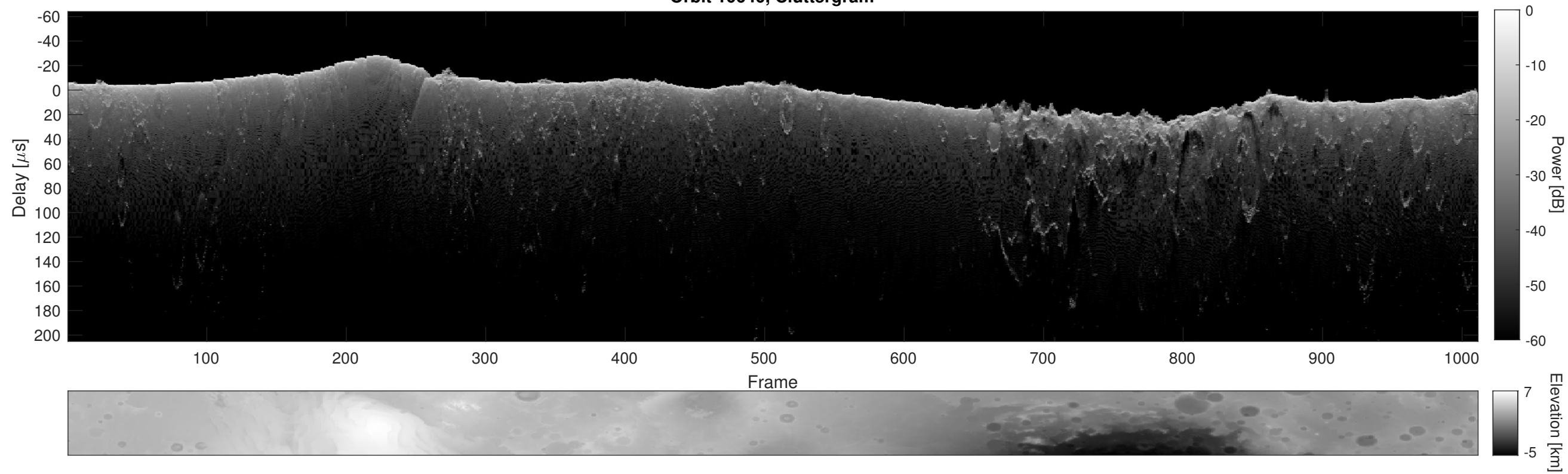
Orbit 10640, Cluttergram
