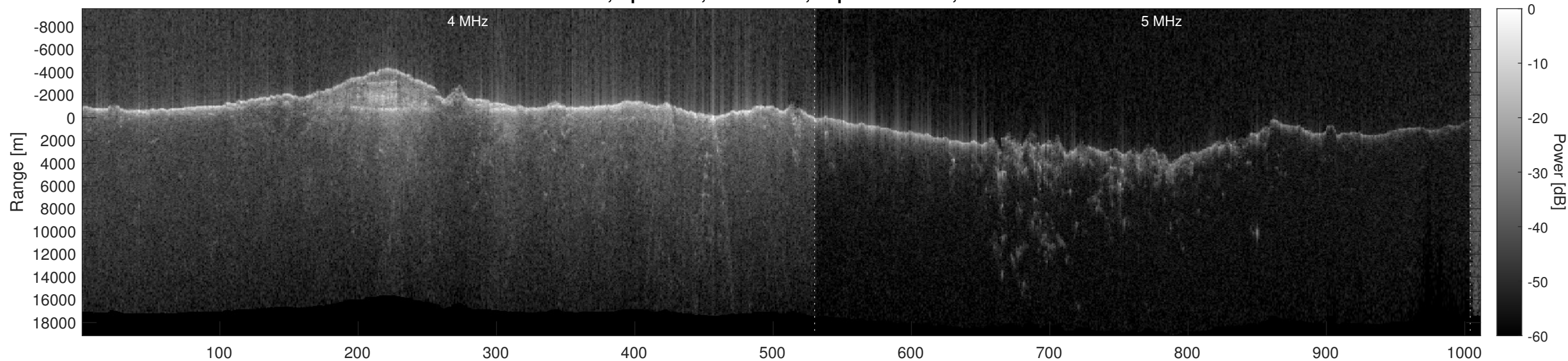
Orbit 10640, Optimized, No Window, Depth-Corrected, Channel 2
