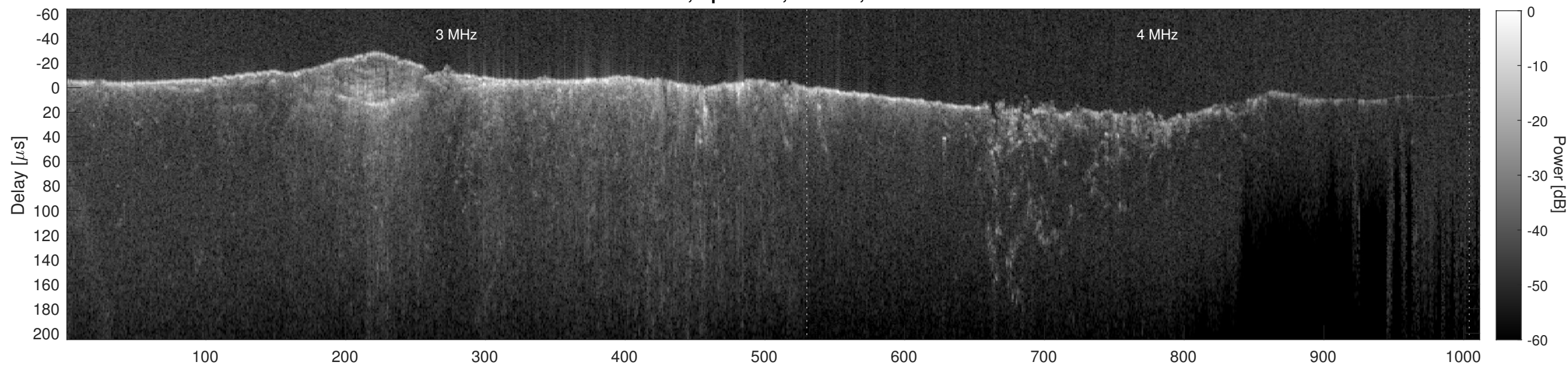
Orbit 10640, Cluttergram
