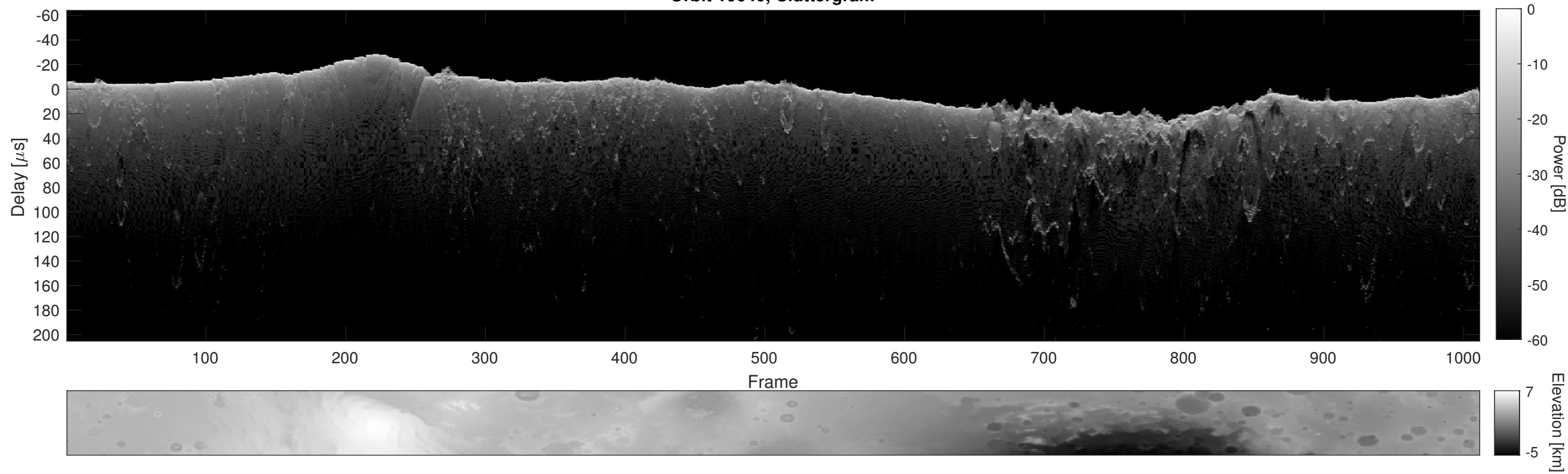
Orbit 10640, Cluttergram
