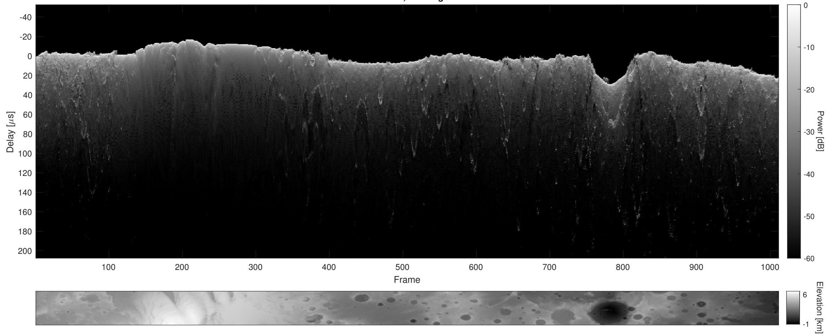
Orbit 10642, Cluttergram
