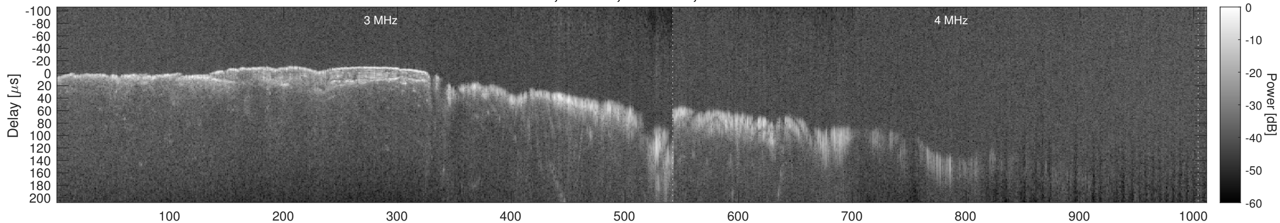
Orbit 10642, Window, Channel 2, Chapman
