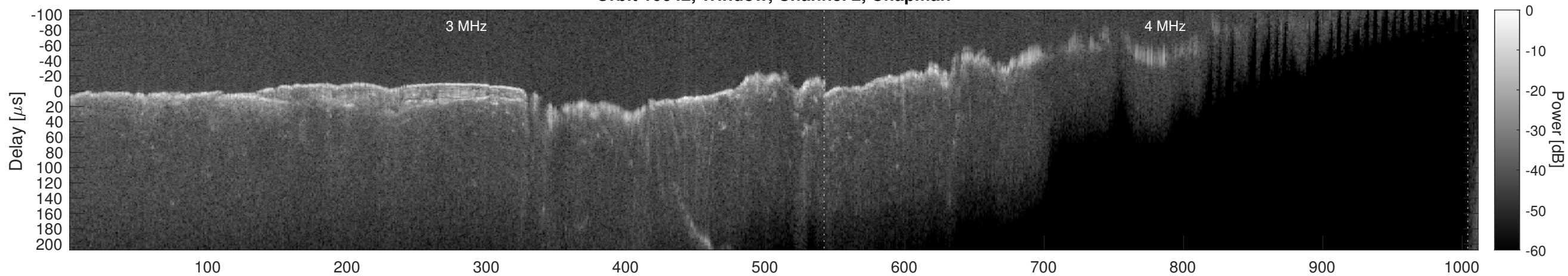
Orbit 10642, Window, Channel 2, Optimized
