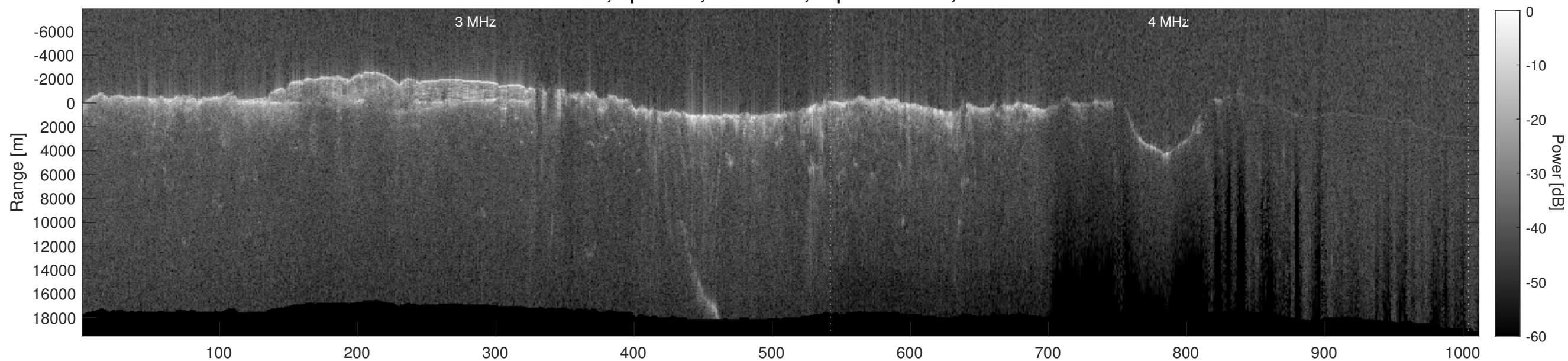
Orbit 10642, Depth-Corrected Cluttergram
