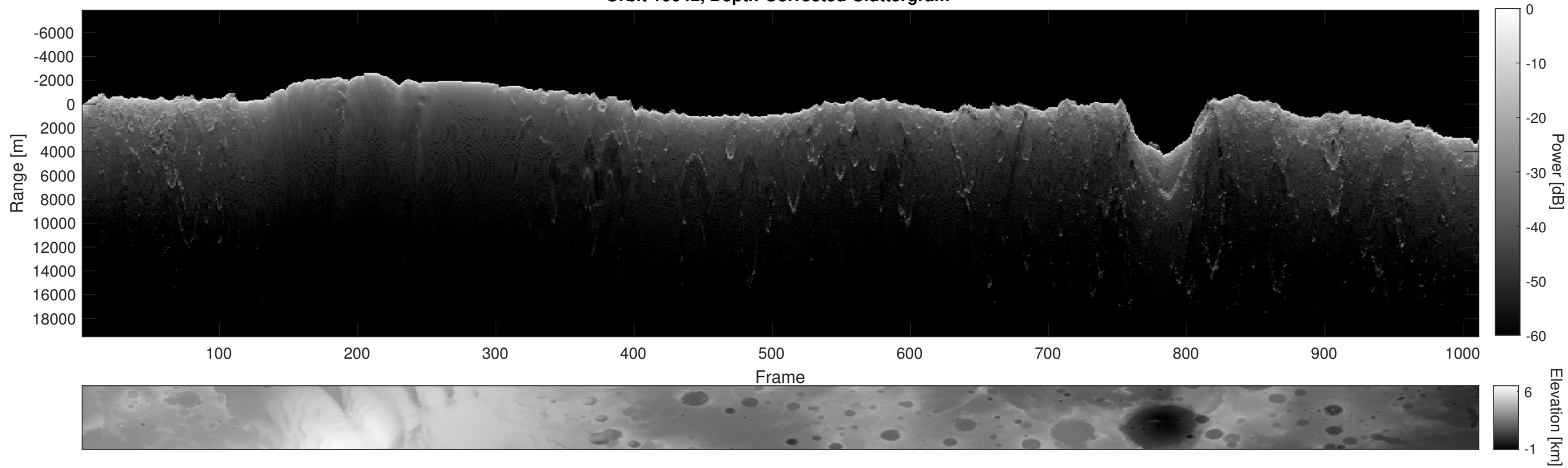
Orbit 10642, Depth-Corrected Cluttergram
