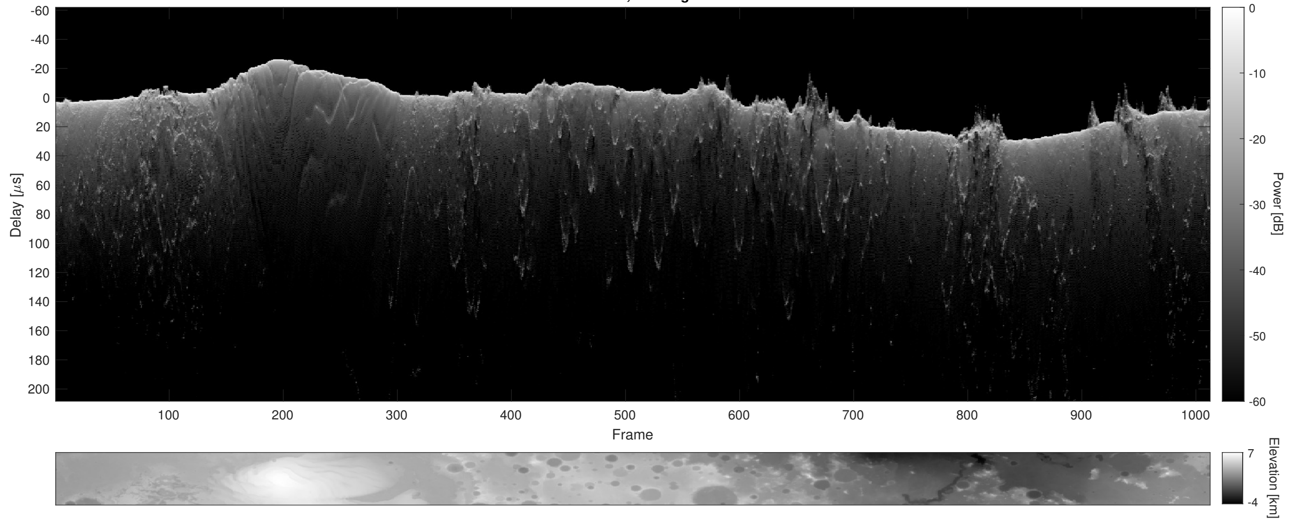
Orbit 10643, Cluttergram
