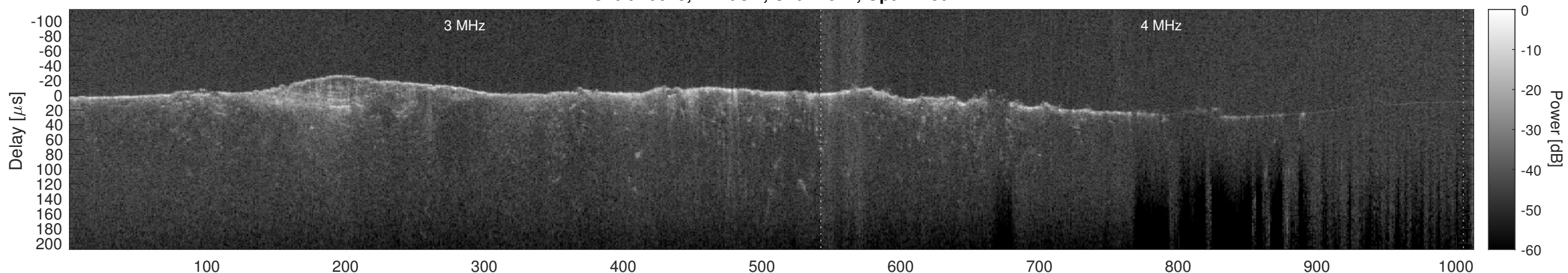
Orbit 10643, Cluttergram
