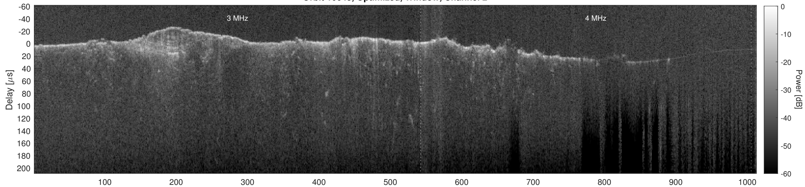
Orbit 10643, Cluttergram
