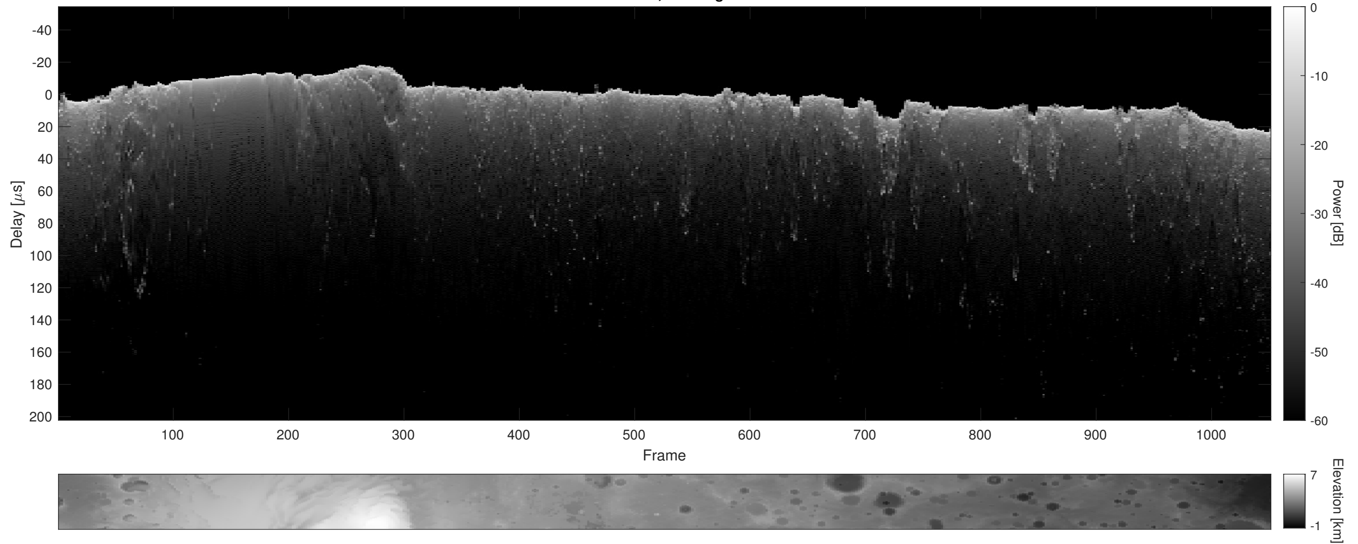
Orbit 10644, Cluttergram
