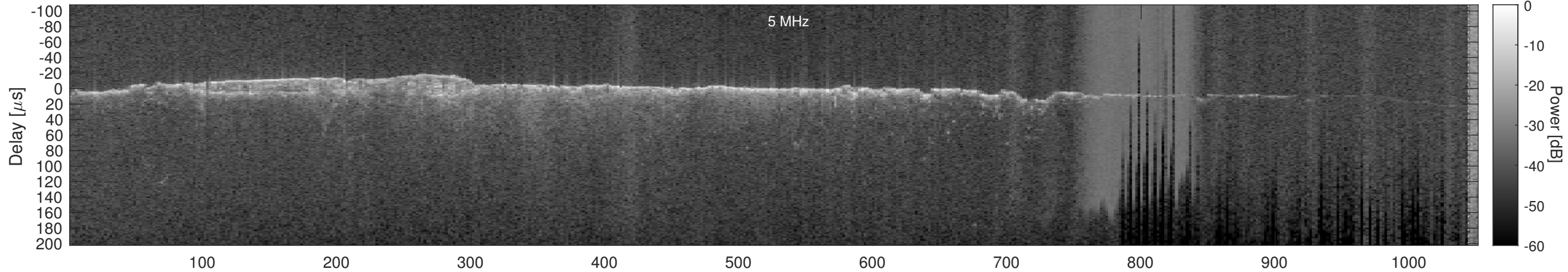
Orbit 10644, Cluttergram
