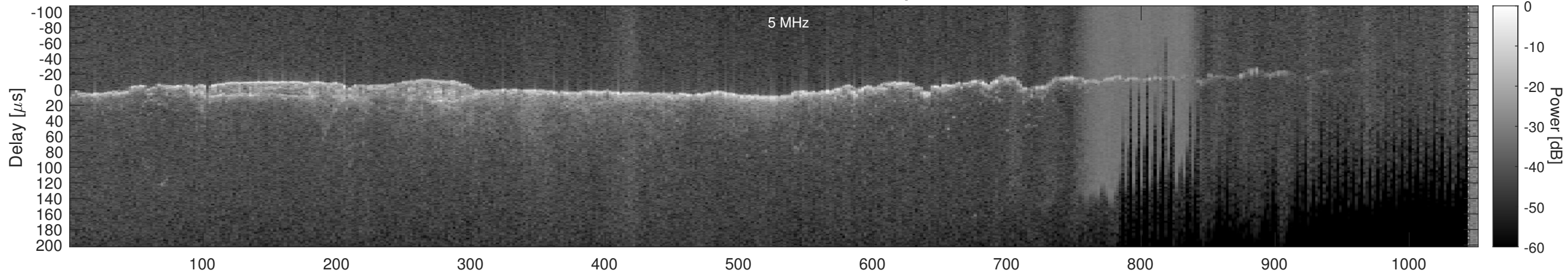
Orbit 10644, Window, Channel 1, Optimized
