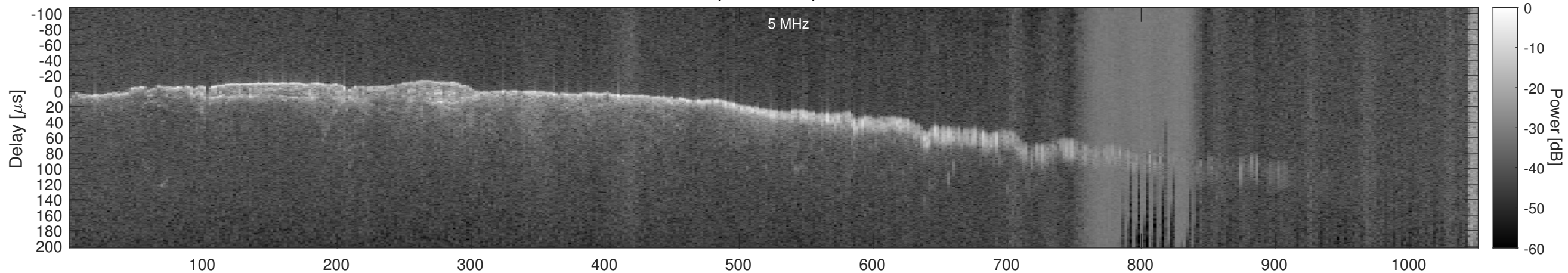
Orbit 10644, Window, Channel 1, Chapman
