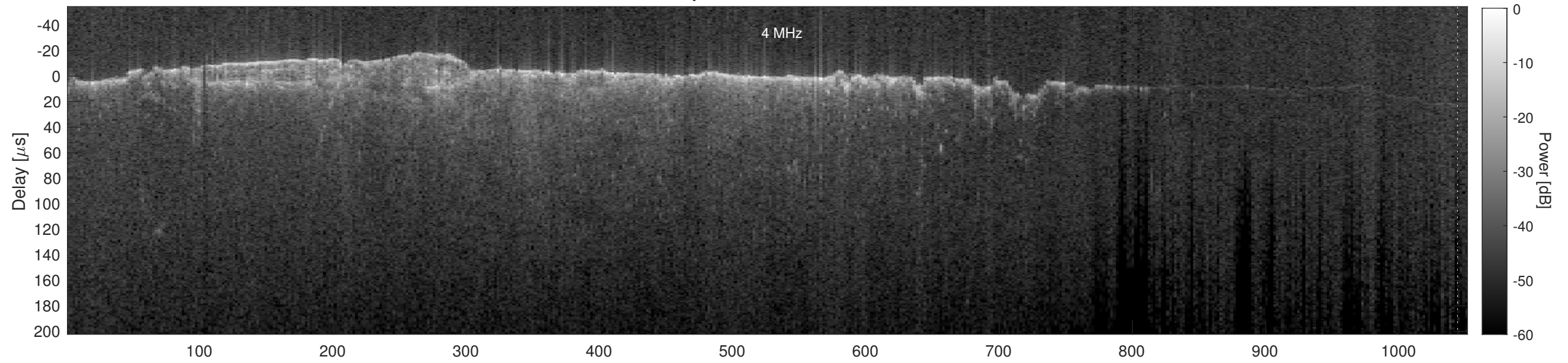
Orbit 10644, Cluttergram
