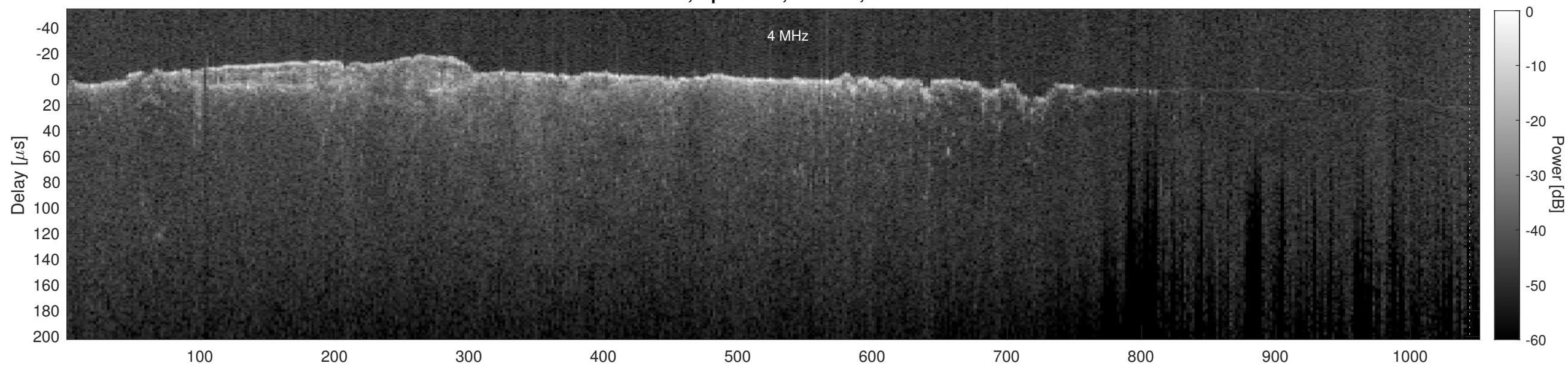
Orbit 10644, Cluttergram
