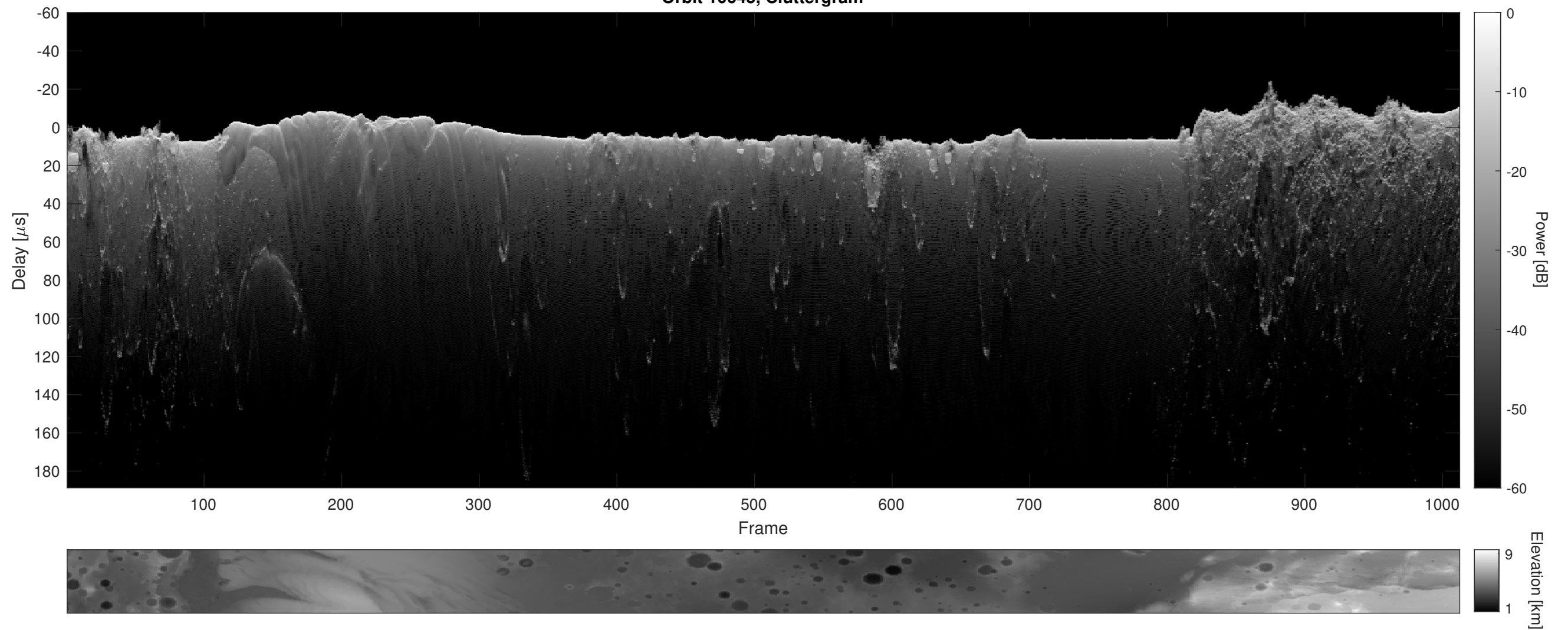
Orbit 10645, Cluttergram
