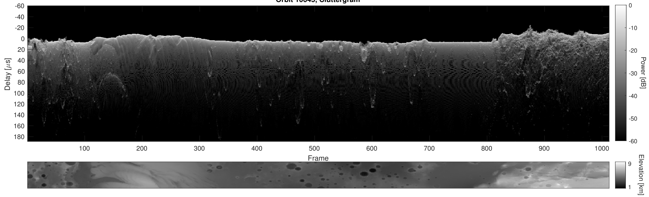
Orbit 10645, Cluttergram
