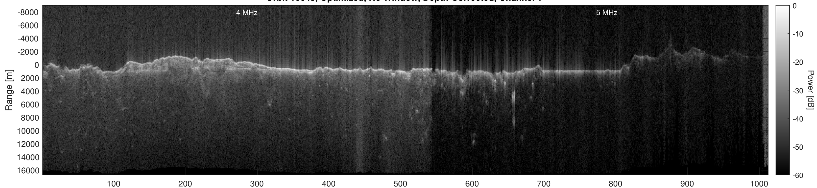
Orbit 10645, Optimized, No Window, Depth-Corrected, Channel 2
