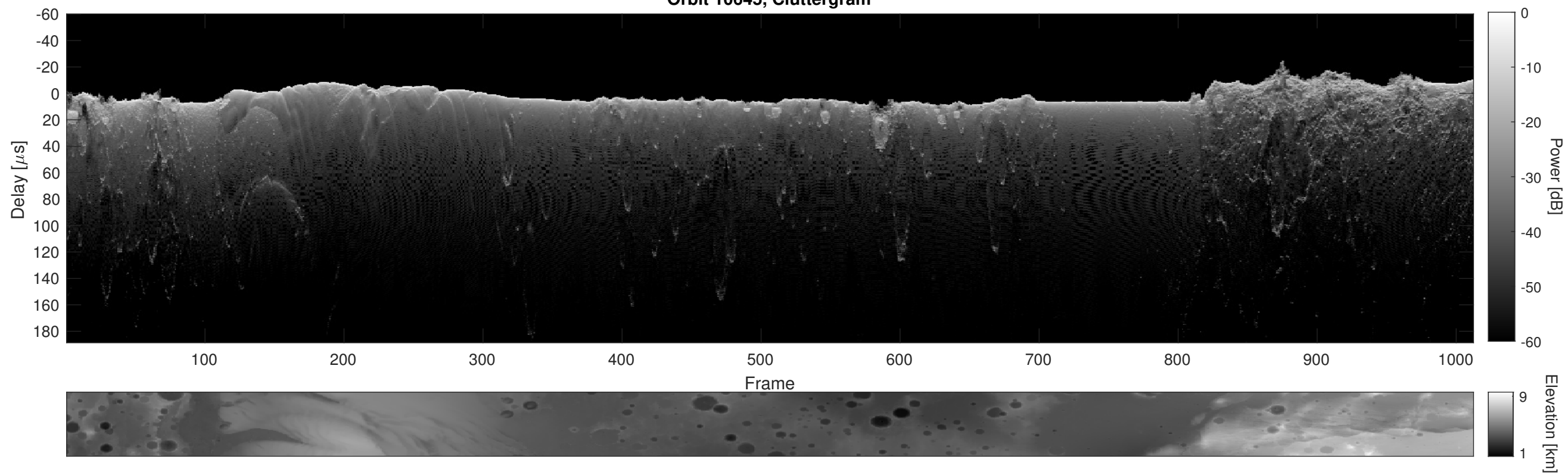
Orbit 10645, Cluttergram
