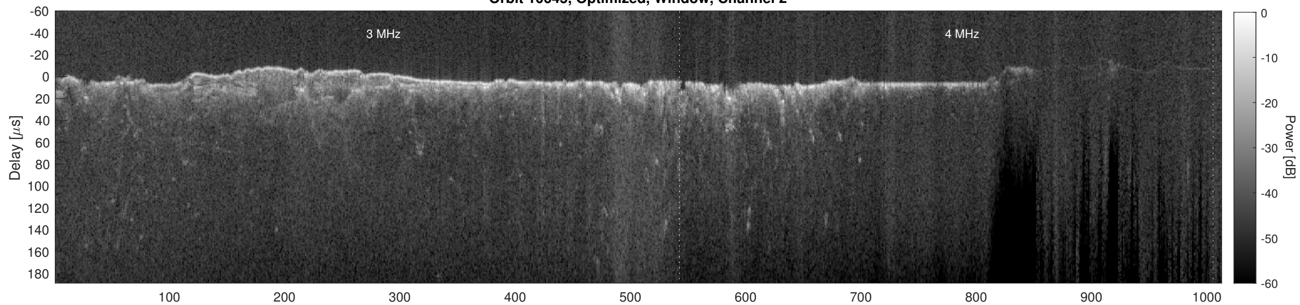
Orbit 10645, Cluttergram
